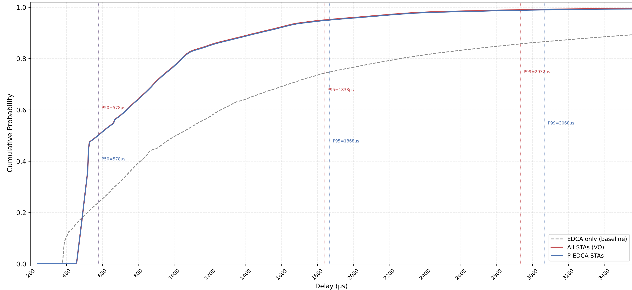
VO Delay CDF — P-EDCA / Legacy / All | CWds=0 × QSRC=0 × PSRC=3 nSta=30, nPedca=30/30, 0.5Mbps, avg of 10 runs
