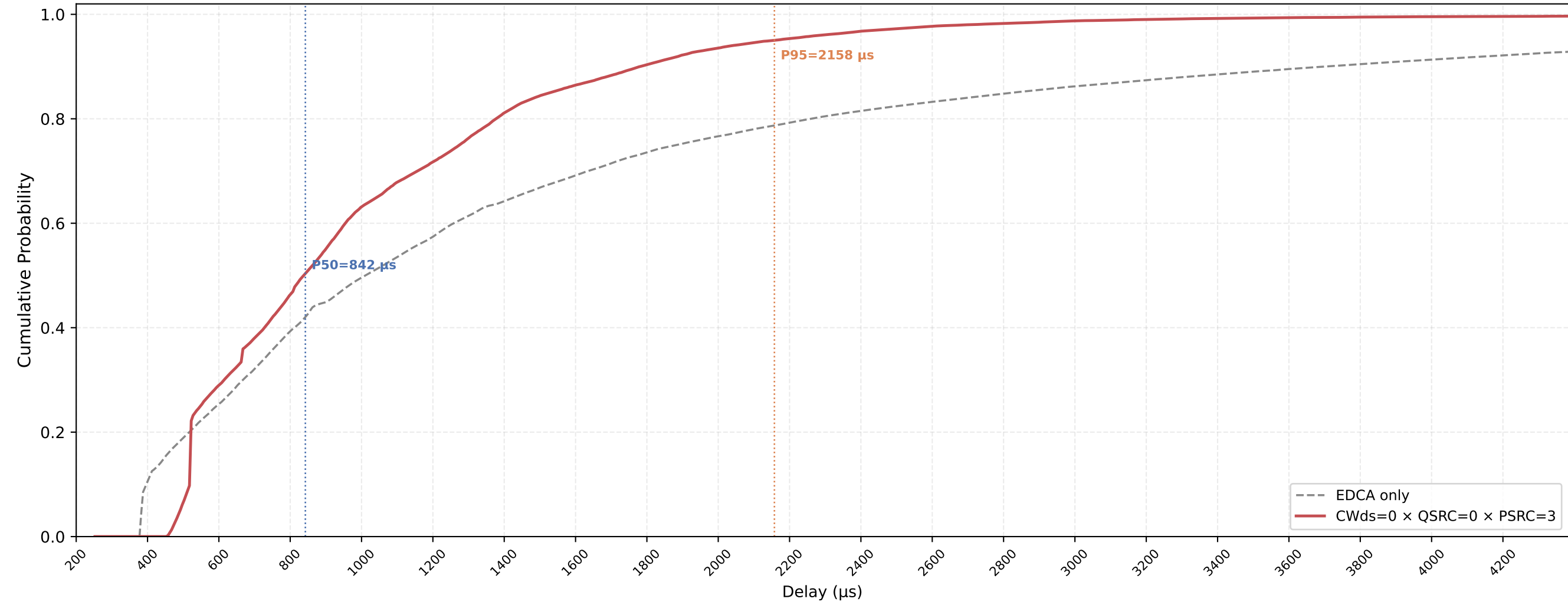
P-EDCA STA VO Delay CDF — CWds=0 × QSRC=0 × PSRC=3 nSta=30, nPedca=5, 0.5Mbps, avg of 10 runs
