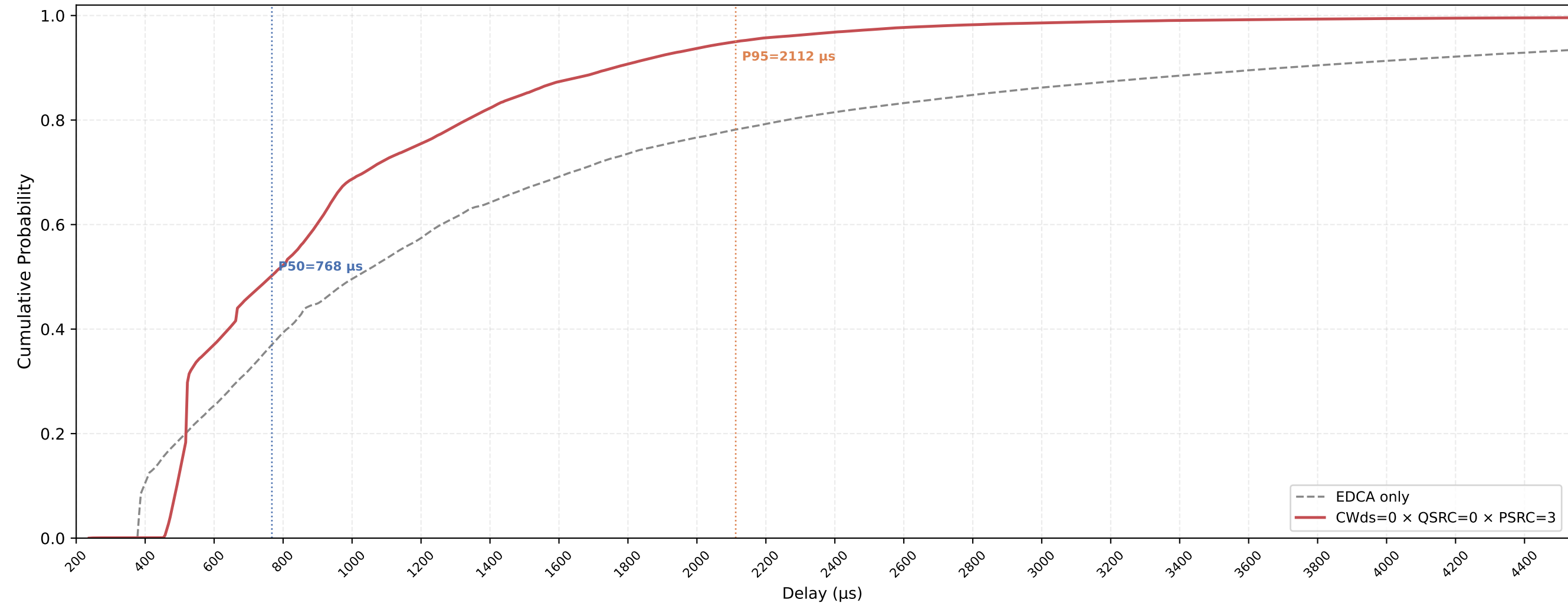
P-EDCA STA VO Delay CDF — CWds=0 × QSRC=0 × PSRC=3 nSta=30, nPedca=15, 0.5Mbps, avg of 10 runs
