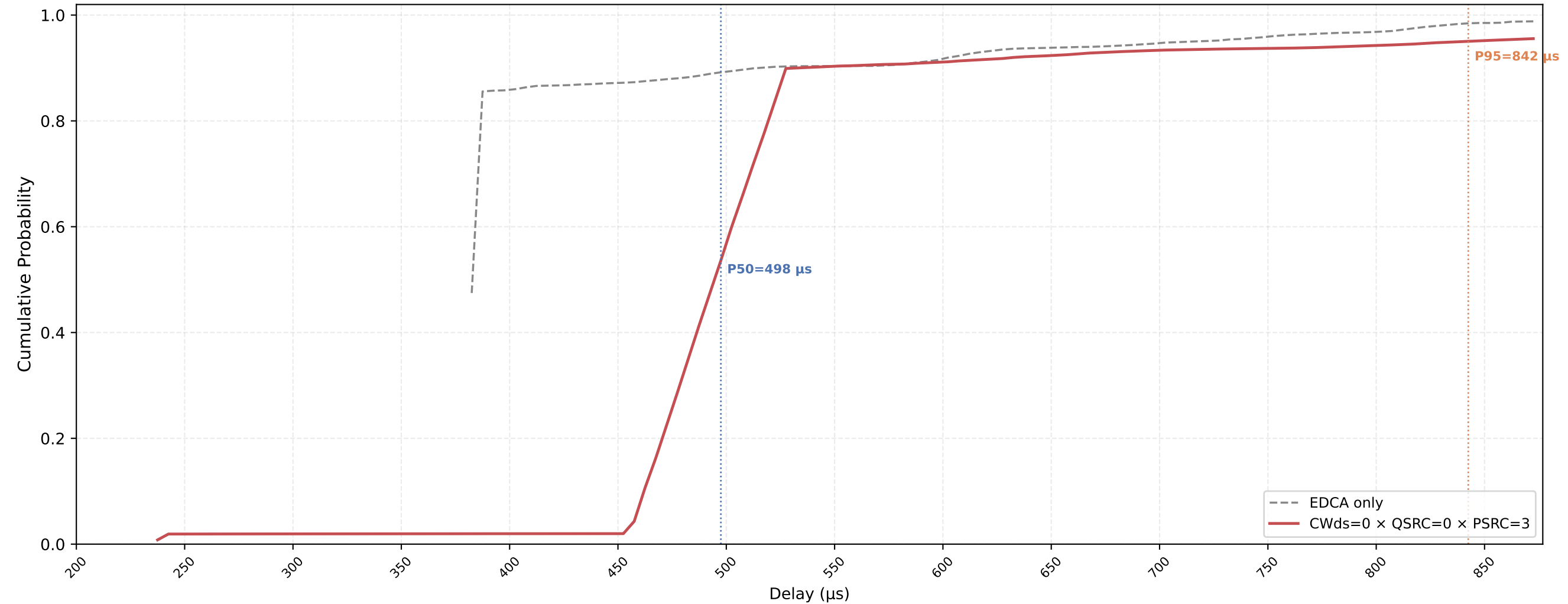
P-EDCA STA VO Delay CDF — CWds=0 × QSRC=0 × PSRC=3 nSta=30, nPedca=30, 0.1Mbps, avg of 10 runs
