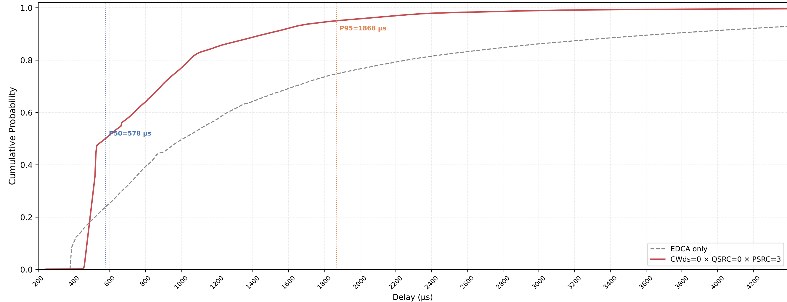
P-EDCA STA VO Delay CDF — CWds=0 × QSRC=0 × PSRC=3 nSta=30, nPedca=30, 0.5Mbps, avg of 10 runs
