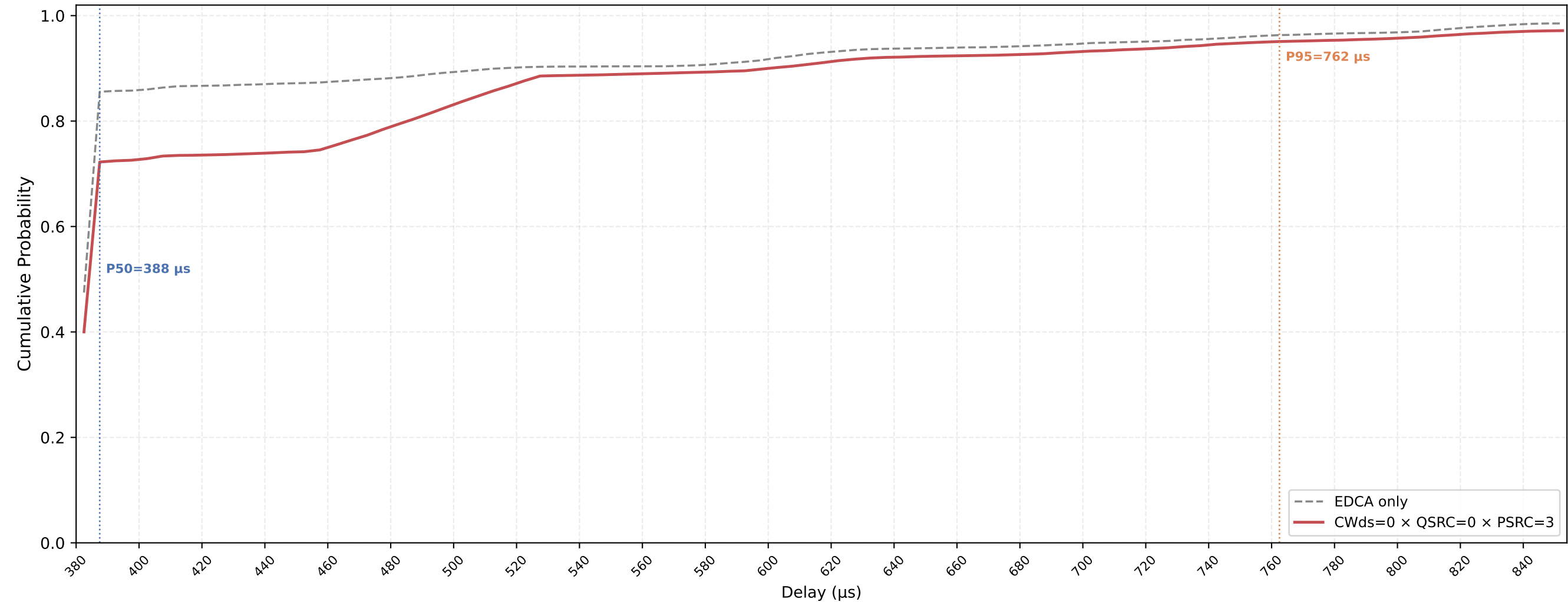
VO (all STAs) Delay CDF — CWds=0 × QSRC=0 × PSRC=3 nSta=30, nPedca=5, 0.1Mbps, avg of 10 runs
