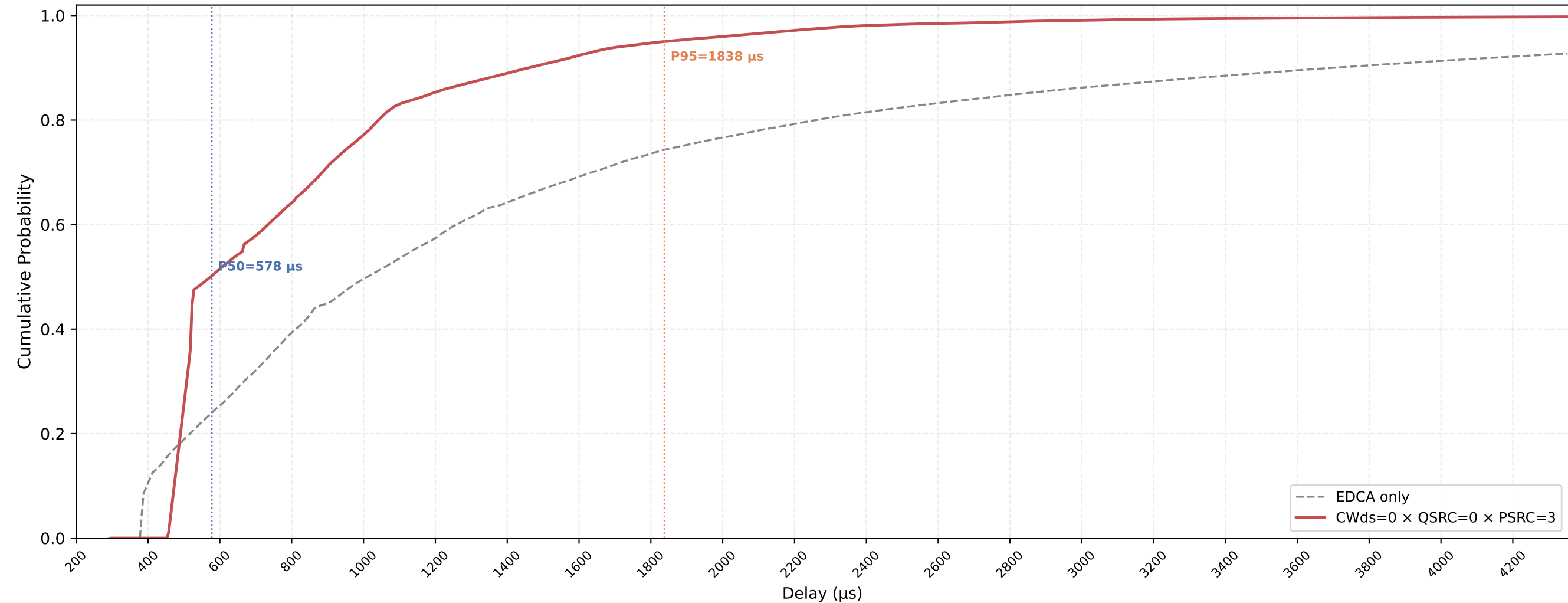
VO (all STAs) Delay CDF — CWds=0 × QSRC=0 × PSRC=3 nSta=30, nPedca=30, 0.5Mbps, avg of 10 runs
