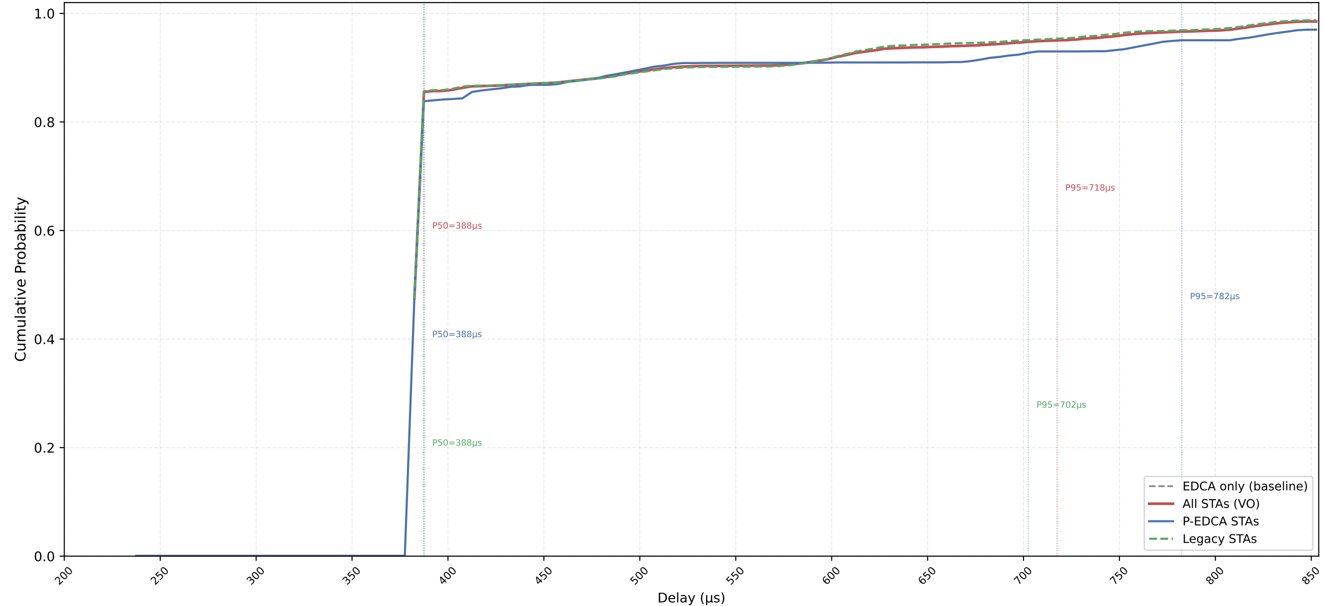
VO Delay CDF — P-EDCA / Legacy / All | CWds=0 × QSRC=1 × PSRC=1 nSta=30, nPedca=5/30, 0.1Mbps, avg of 10 runs
