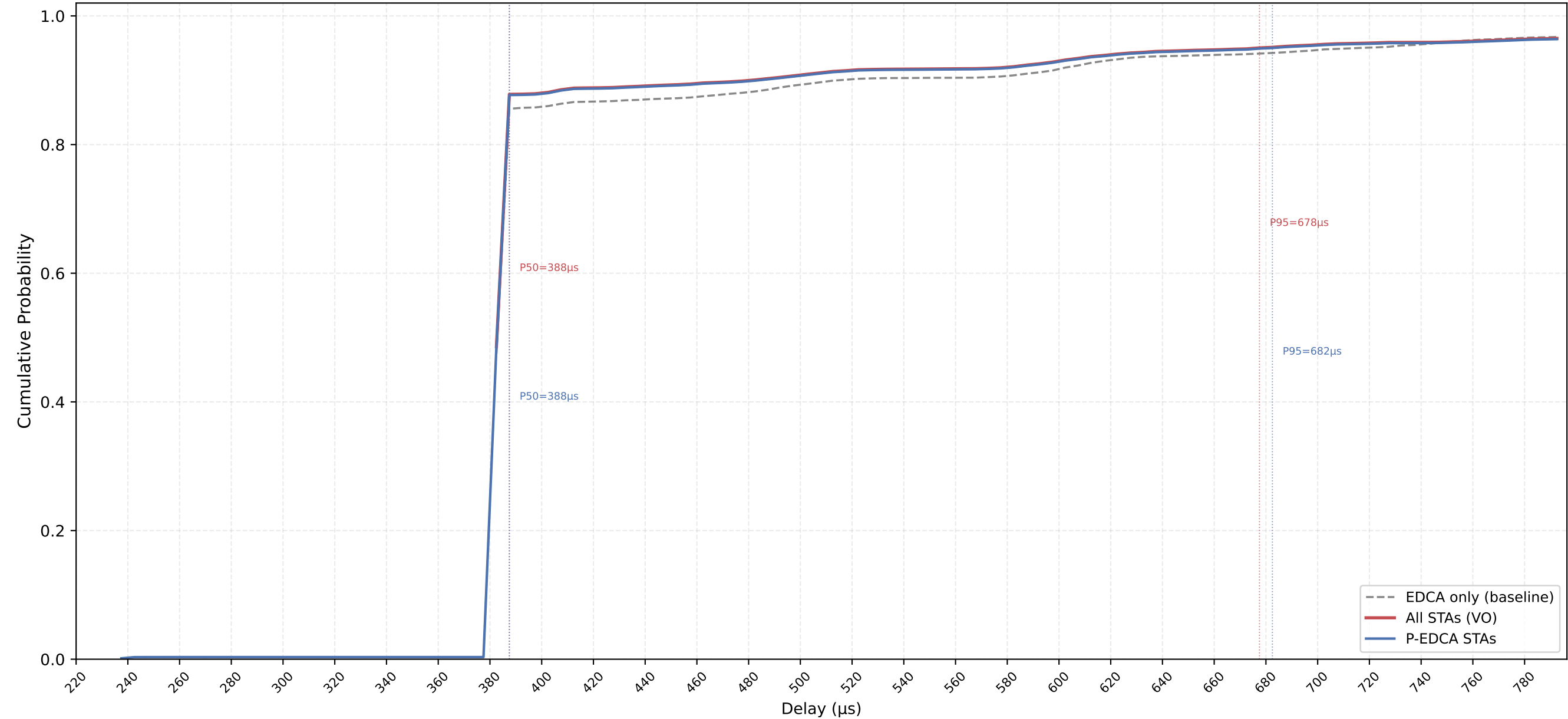
VO Delay CDF — P-EDCA / Legacy / All | CWds=0 × QSRC=1 × PSRC=1 nSta=30, nPedca=30/30, 0.1Mbps, avg of 10 runs
