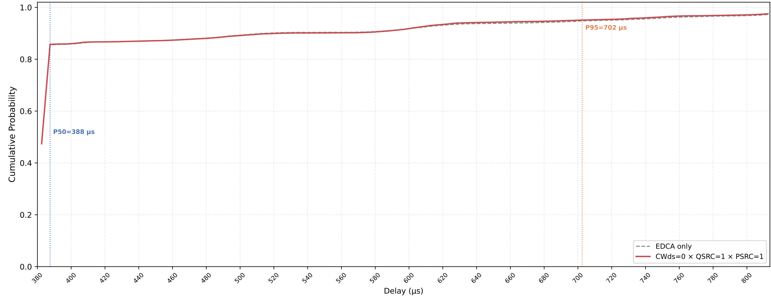
Legacy STA VO Delay CDF — CWds=0 × QSRC=1 × PSRC=1 nSta=30, nPedca=5, 0.1Mbps, avg of 10 runs
