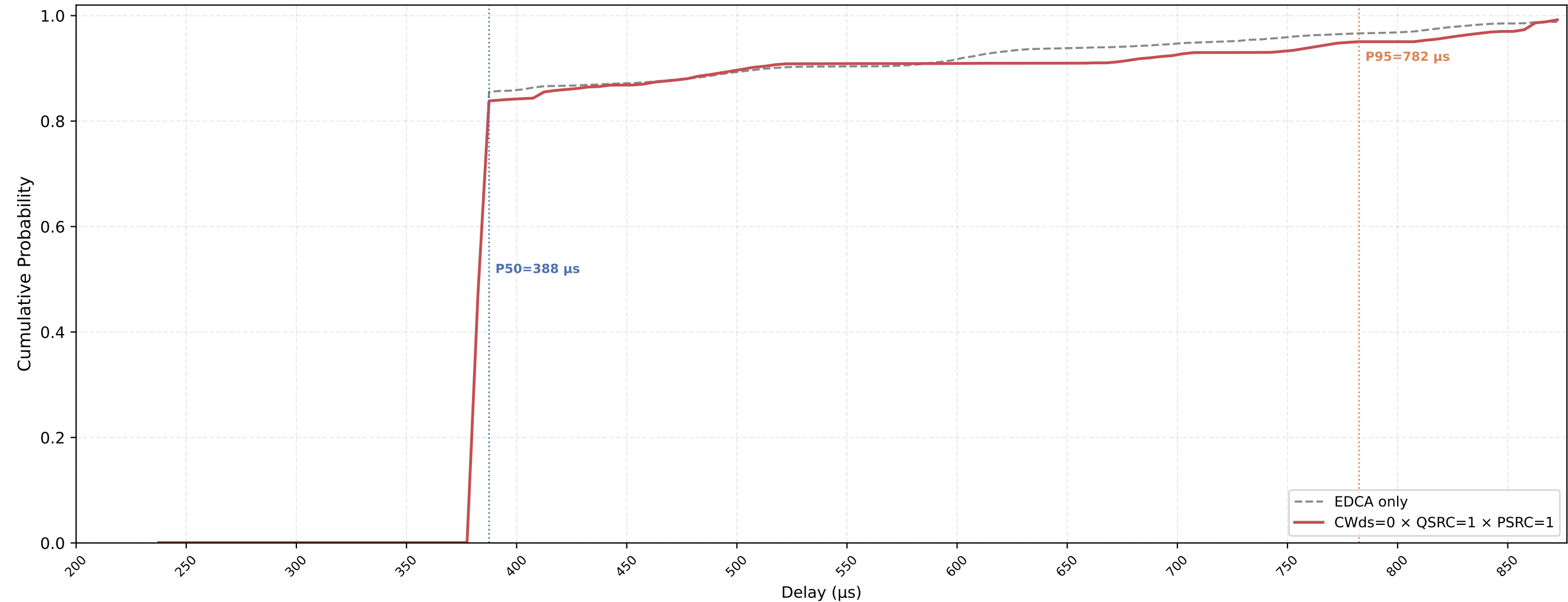
P-EDCA STA VO Delay CDF — CWds=0 × QSRC=1 × PSRC=1 nSta=30, nPedca=5, 0.1Mbps, avg of 10 runs
