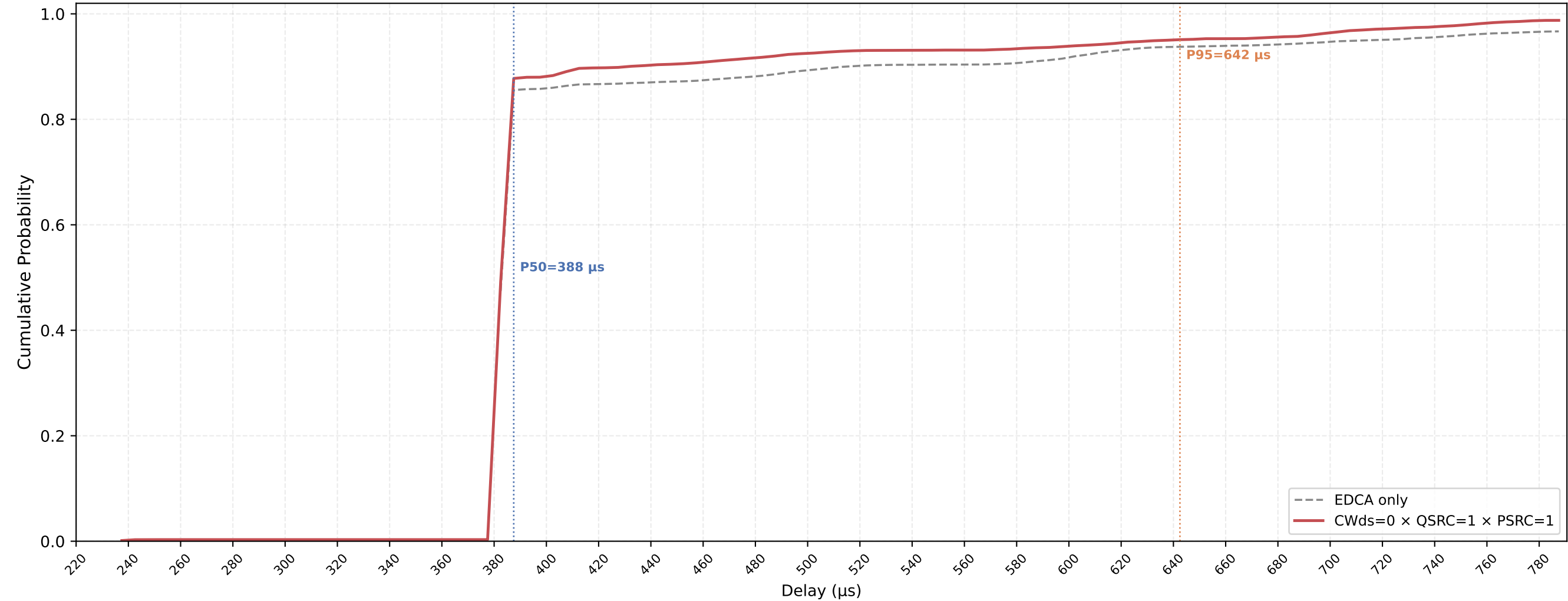
P-EDCA STA VO Delay CDF — CWds=0 × QSRC=1 × PSRC=1 nSta=30, nPedca=15, 0.1Mbps, avg of 10 runs
