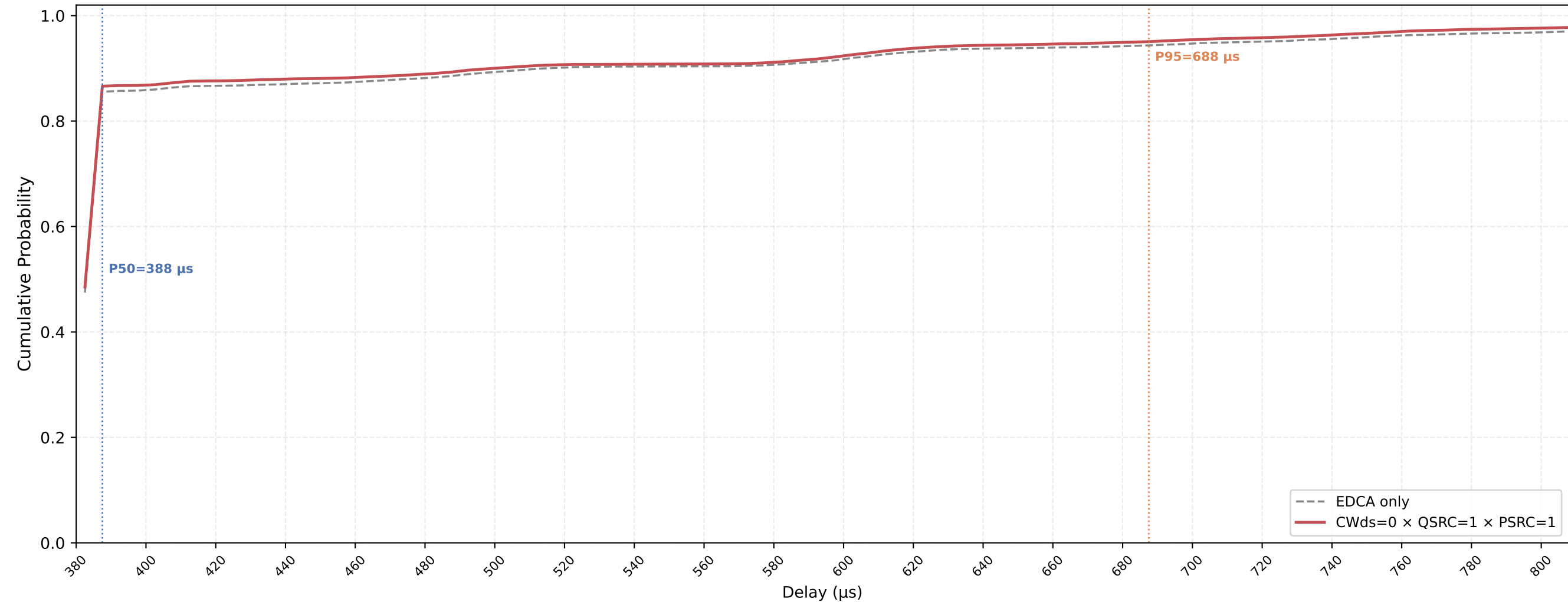
VO (all STAs) Delay CDF — CWds=0 × QSRC=1 × PSRC=1 nSta=30, nPedca=15, 0.1Mbps, avg of 10 runs
