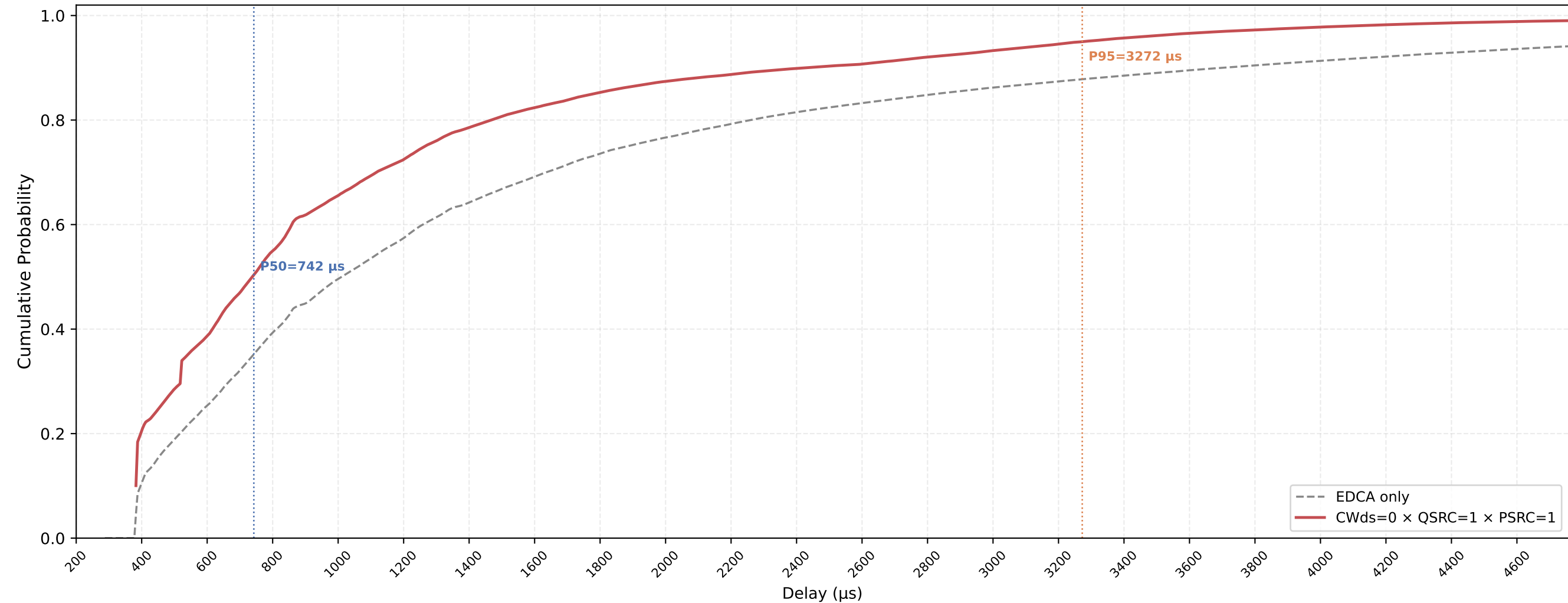
VO (all STAs) Delay CDF — CWds=0 × QSRC=1 × PSRC=1 nSta=30, nPedca=30, 0.5Mbps, avg of 10 runs
