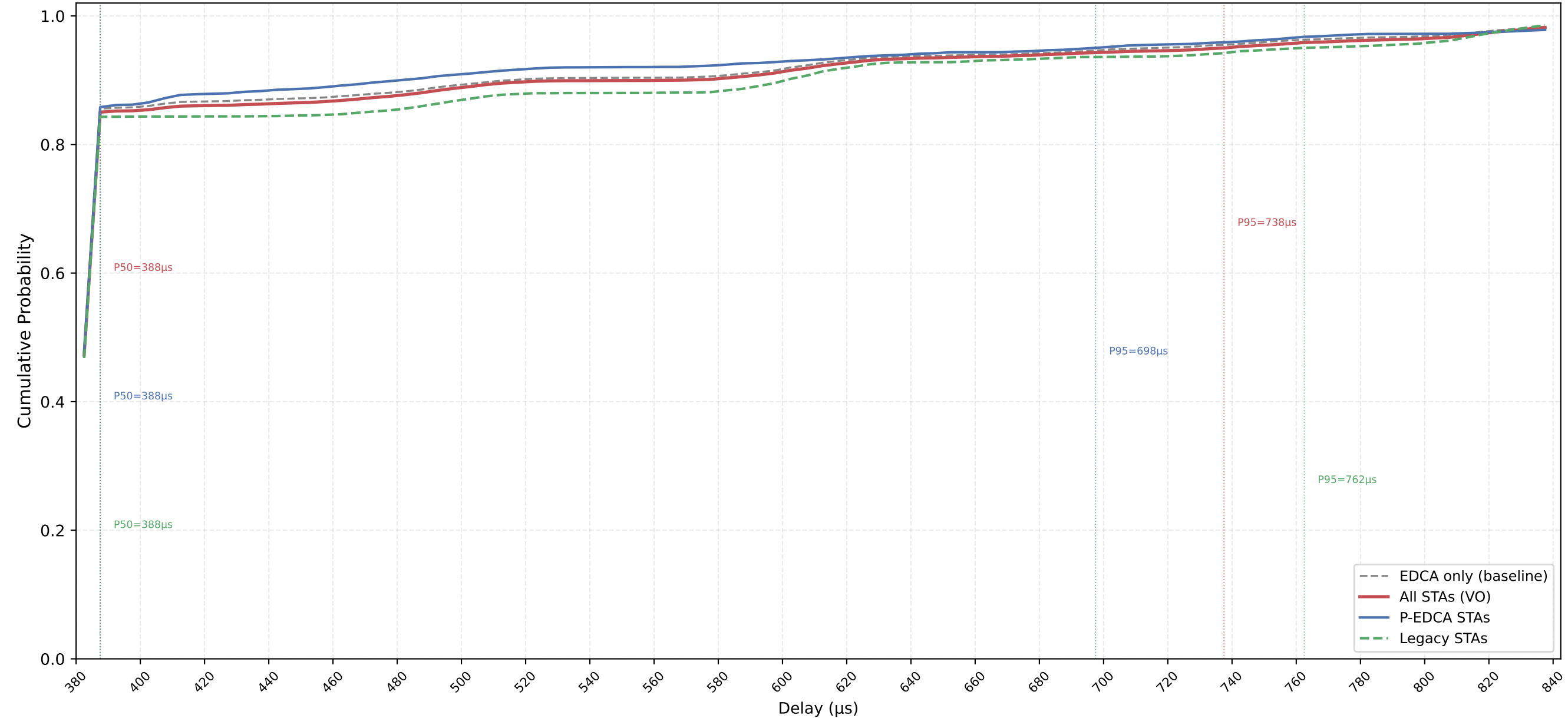
VO Delay CDF — P-EDCA / Legacy / All | CWds=0 × QSRC=1 × PSRC=2 nSta=30, nPedca=15/30, 0.1Mbps, avg of 10 runs
