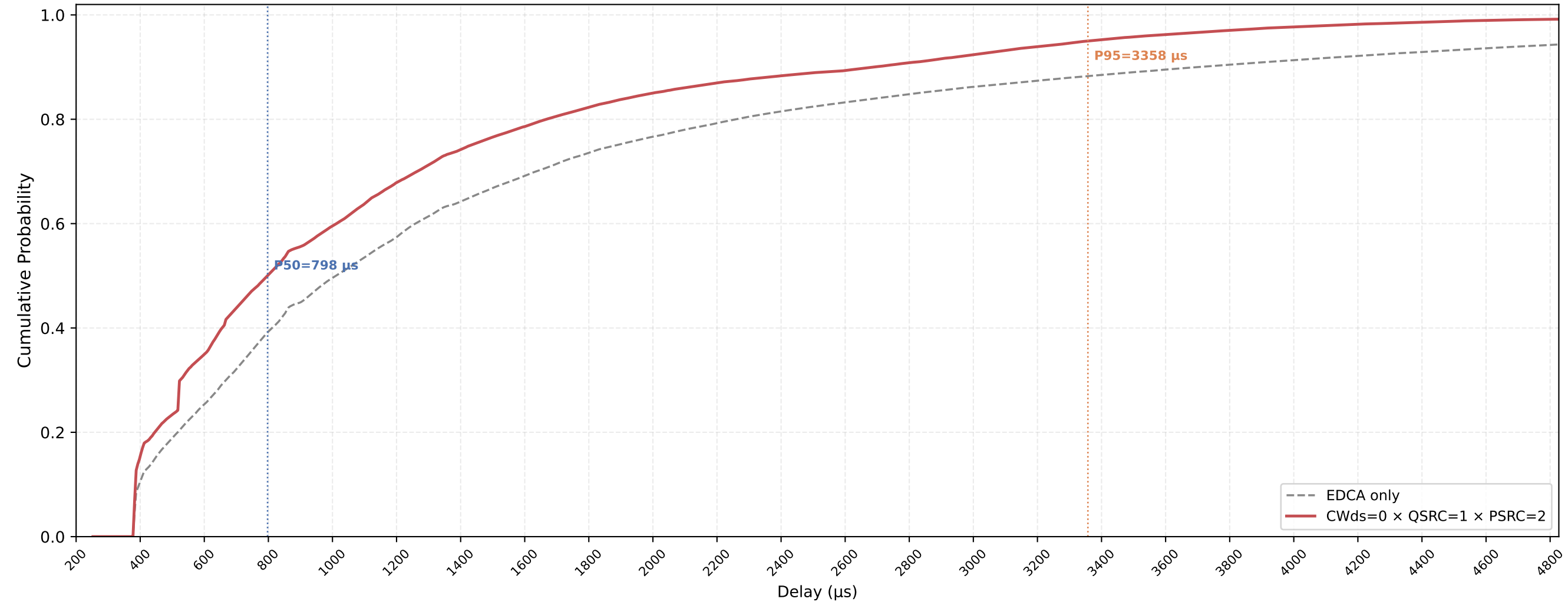
P-EDCA STA VO Delay CDF — CWds=0 × QSRC=1 × PSRC=2 nSta=30, nPedca=15, 0.5Mbps, avg of 10 runs
