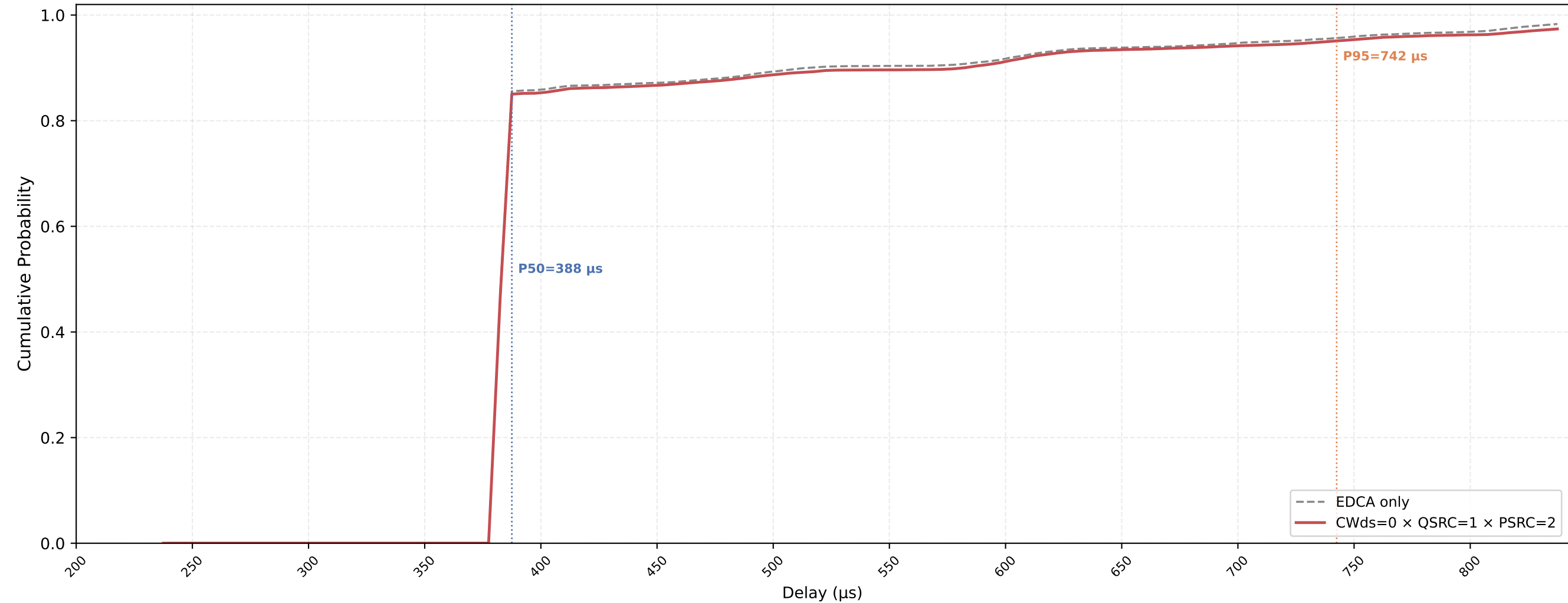
P-EDCA STA VO Delay CDF — CWds=0 × QSRC=1 × PSRC=2 nSta=30, nPedca=30, 0.1Mbps, avg of 10 runs
