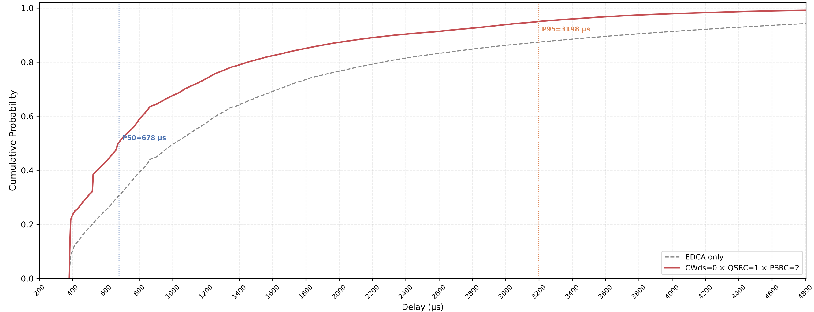
VO (all STAs) Delay CDF — CWds=0 × QSRC=1 × PSRC=2 nSta=30, nPedca=30, 0.5Mbps, avg of 10 runs
