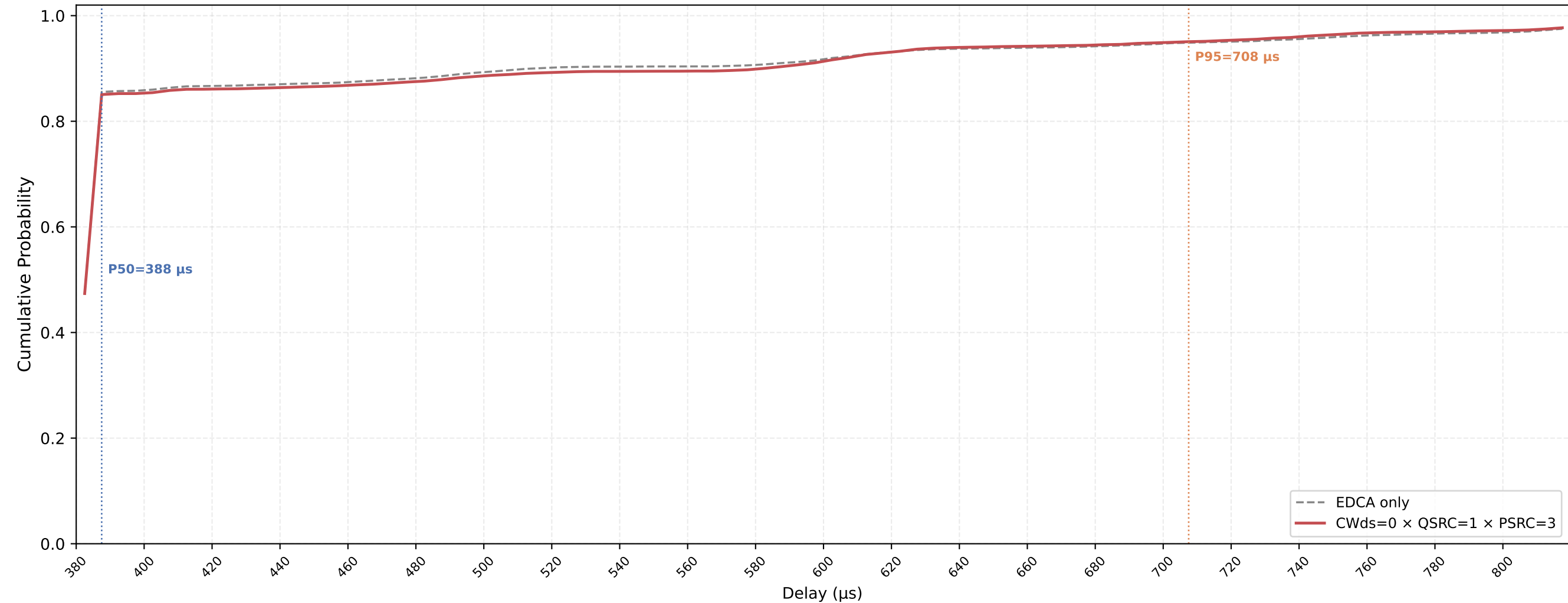
Legacy STA VO Delay CDF — CWds=0 × QSRC=1 × PSRC=3 nSta=30, nPedca=5, 0.1Mbps, avg of 10 runs
