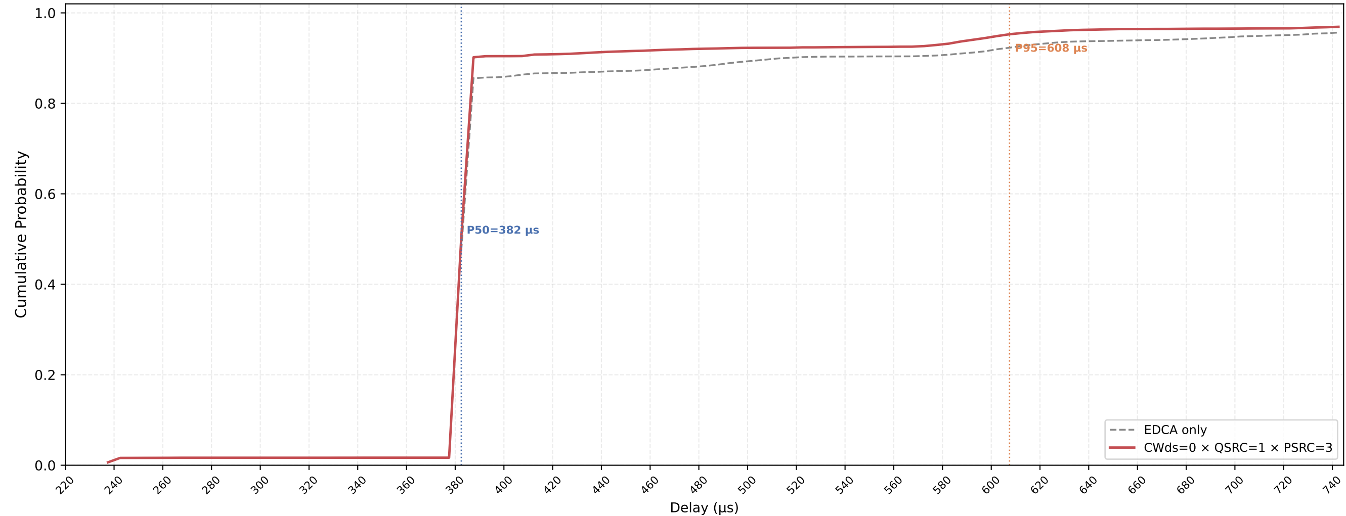
P-EDCA STA VO Delay CDF — CWds=0 × QSRC=1 × PSRC=3 nSta=30, nPedca=30, 0.1Mbps, avg of 10 runs
