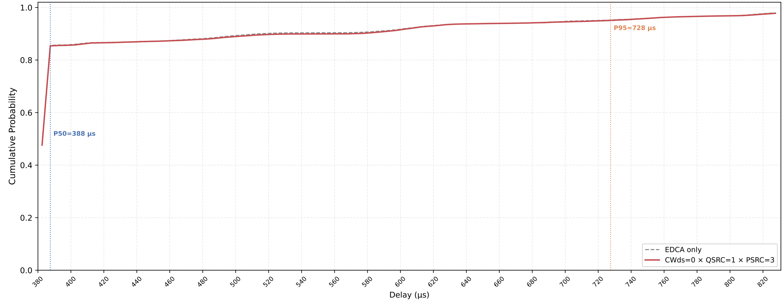
VO (all STAs) Delay CDF — CWds=0 × QSRC=1 × PSRC=3 nSta=30, nPedca=5, 0.1Mbps, avg of 10 runs
