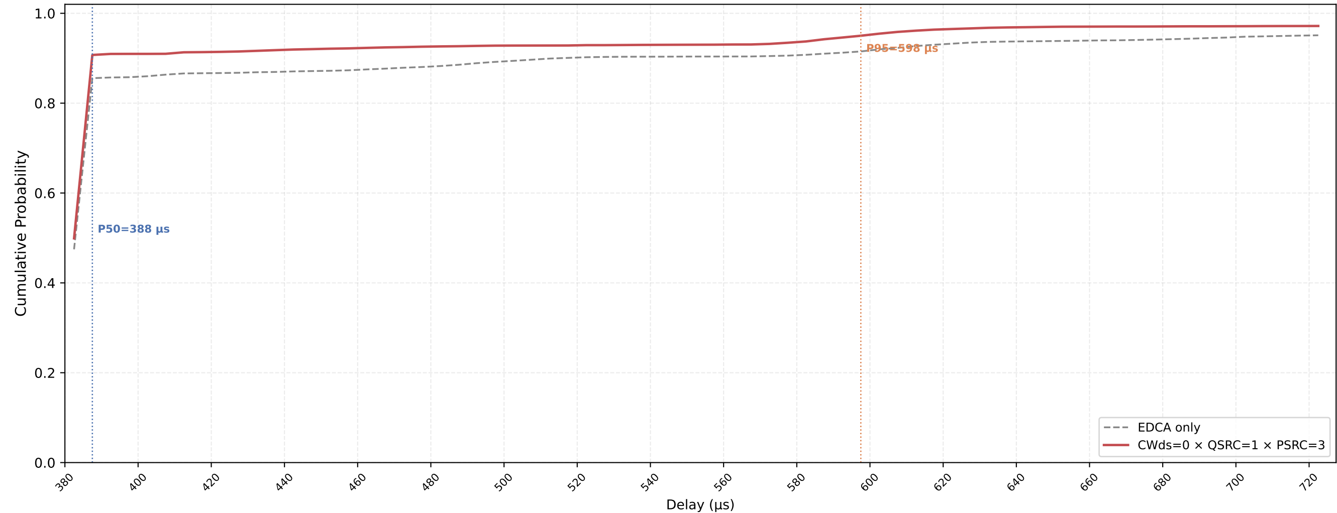
VO (all STAs) Delay CDF — CWds=0 × QSRC=1 × PSRC=3 nSta=30, nPedca=30, 0.1Mbps, avg of 10 runs
