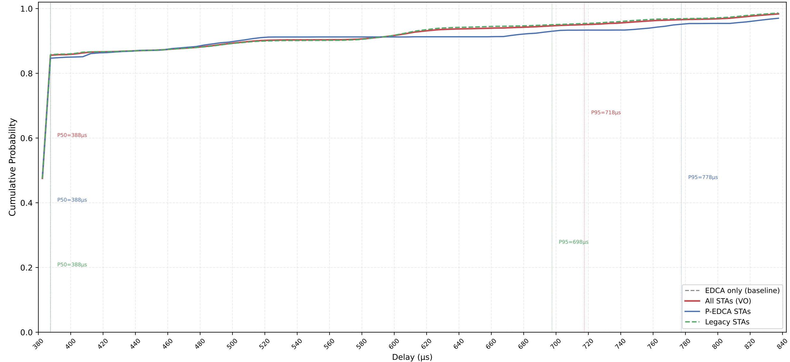
VO Delay CDF — P-EDCA / Legacy / All | CWds=0 × QSRC=2 × PSRC=1 nSta=30, nPedca=5/30, 0.1Mbps, avg of 10 runs
