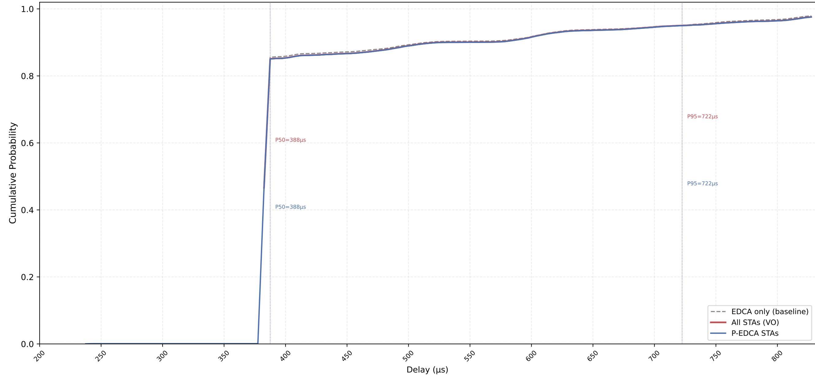
VO Delay CDF — P-EDCA / Legacy / All | CWds=0 × QSRC=2 × PSRC=1 nSta=30, nPedca=30/30, 0.1Mbps, avg of 10 runs
