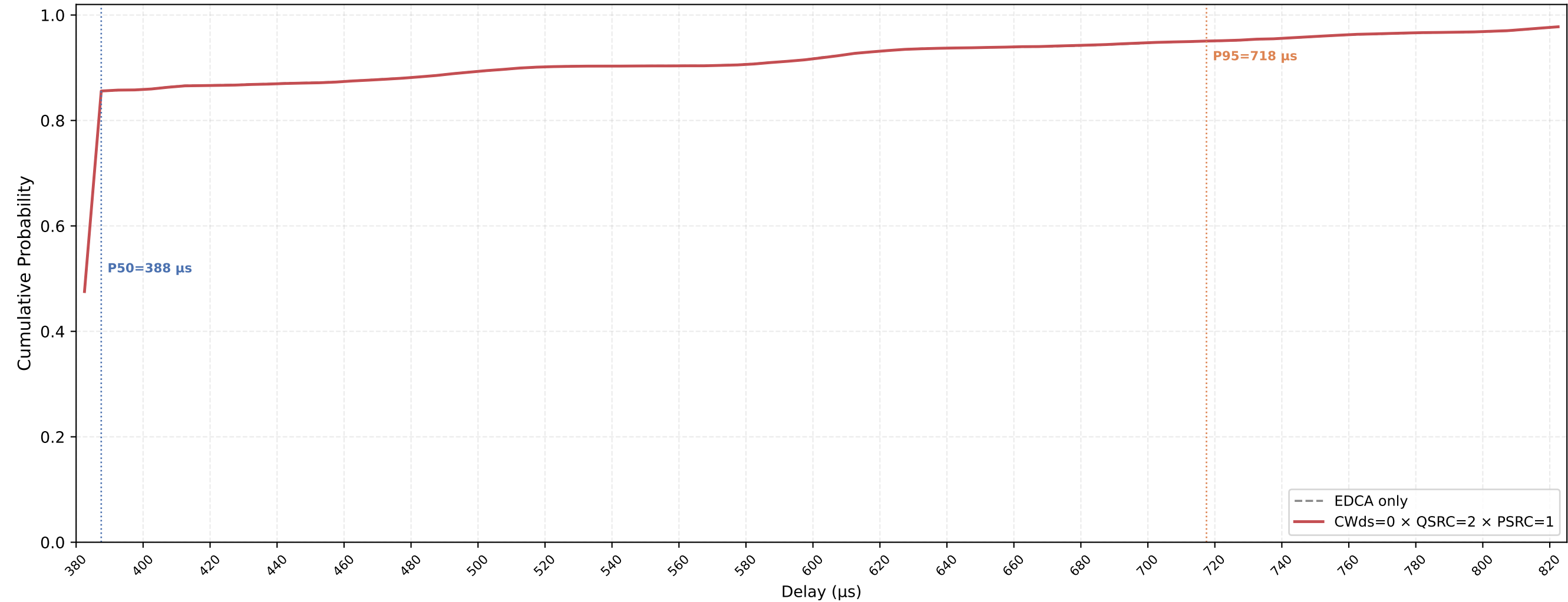
VO (all STAs) Delay CDF — CWds=0 × QSRC=2 × PSRC=1 nSta=30, nPedca=5, 0.1Mbps, avg of 10 runs
