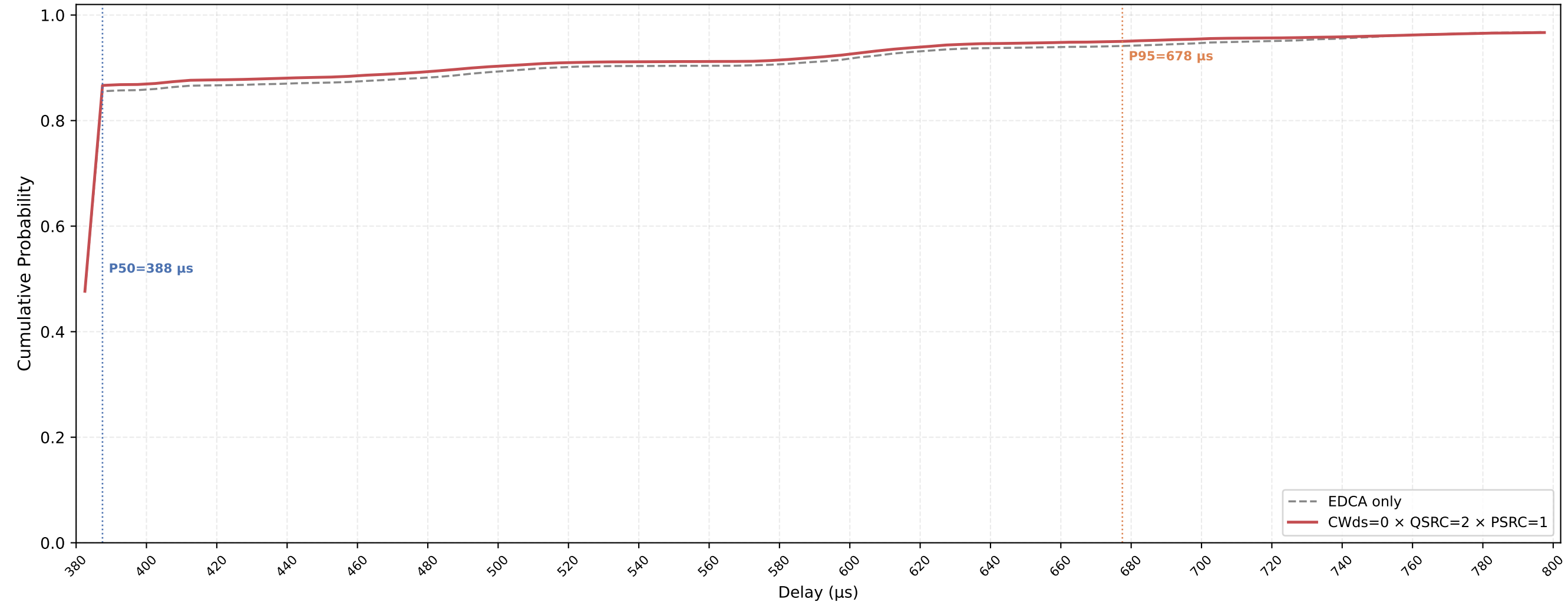
VO (all STAs) Delay CDF — CWds=0 × QSRC=2 × PSRC=1 nSta=30, nPedca=15, 0.1Mbps, avg of 10 runs
