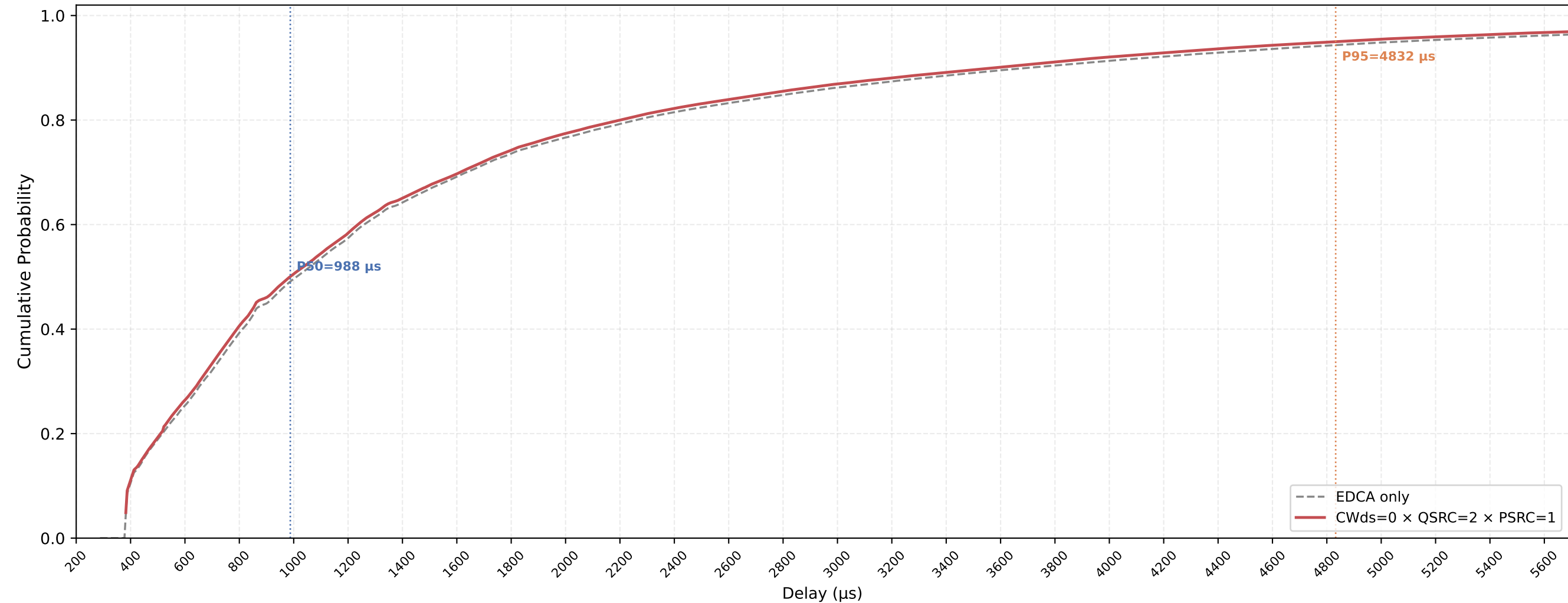
VO (all STAs) Delay CDF — CWds=0 × QSRC=2 × PSRC=1 nSta=30, nPedca=15, 0.5Mbps, avg of 10 runs
