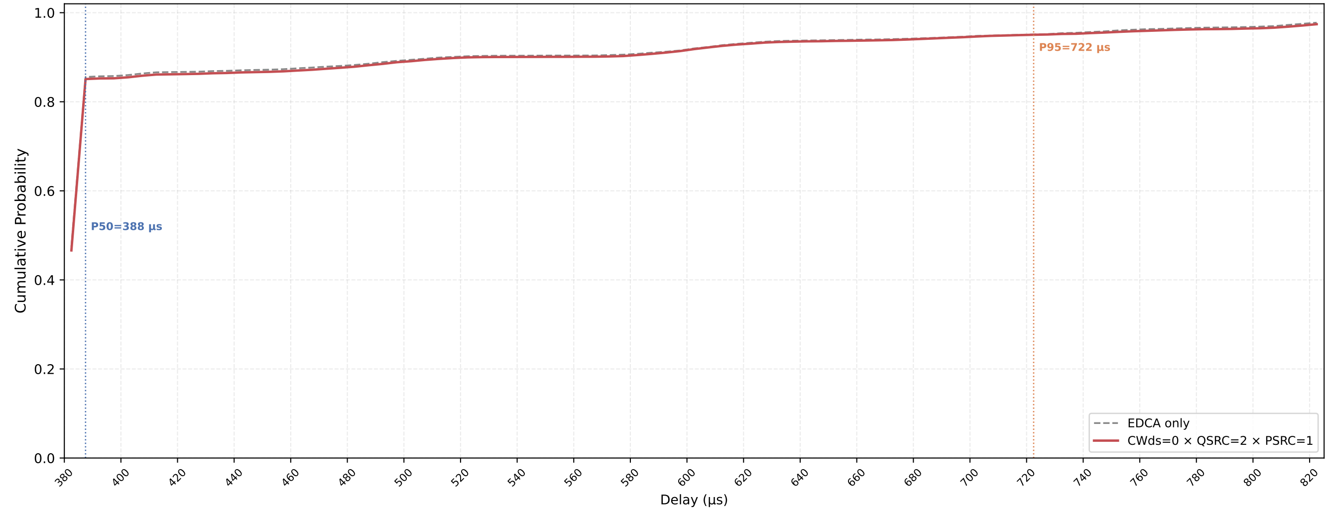
VO (all STAs) Delay CDF — CWds=0 × QSRC=2 × PSRC=1 nSta=30, nPedca=30, 0.1Mbps, avg of 10 runs
