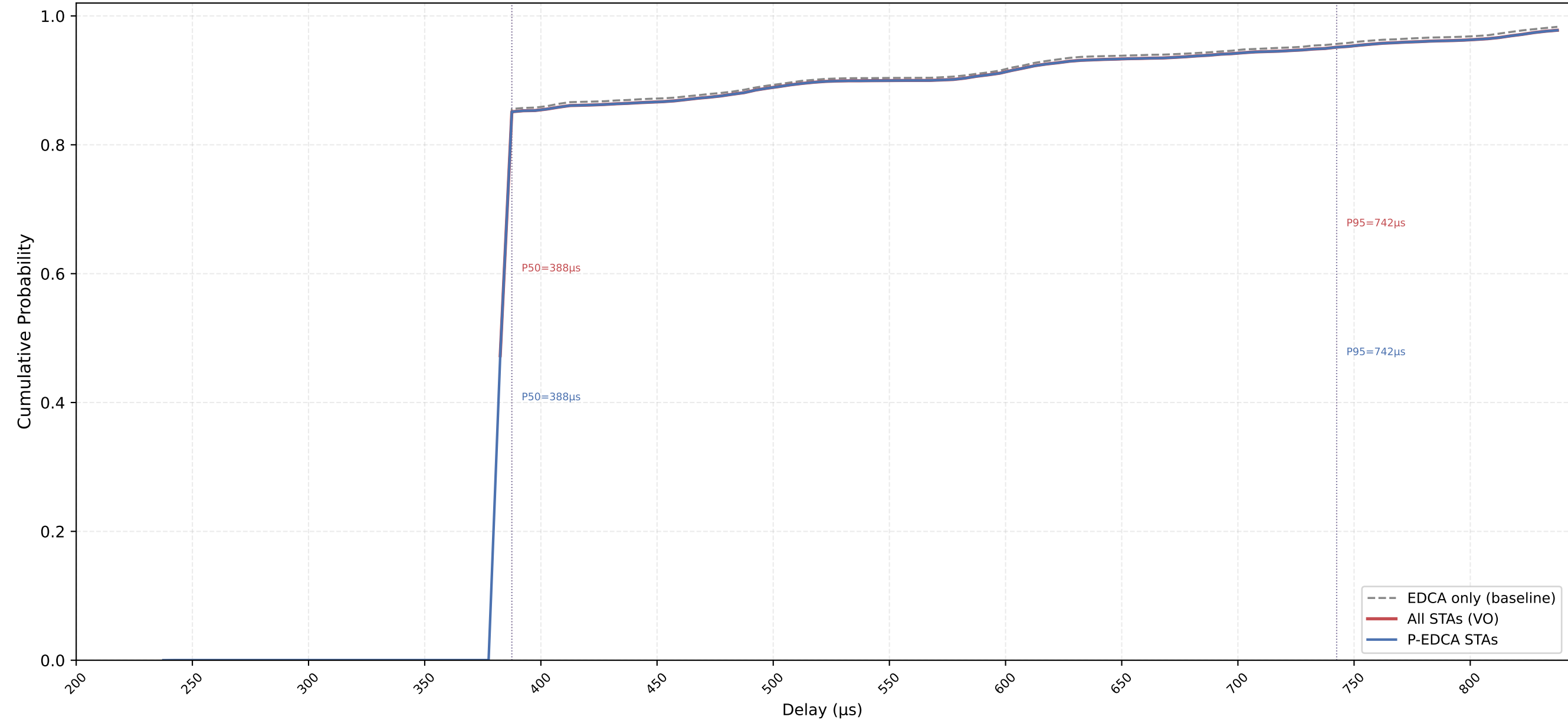
VO Delay CDF — P-EDCA / Legacy / All | CWds=0 × QSRC=2 × PSRC=2 nSta=30, nPedca=30/30, 0.1Mbps, avg of 10 runs
