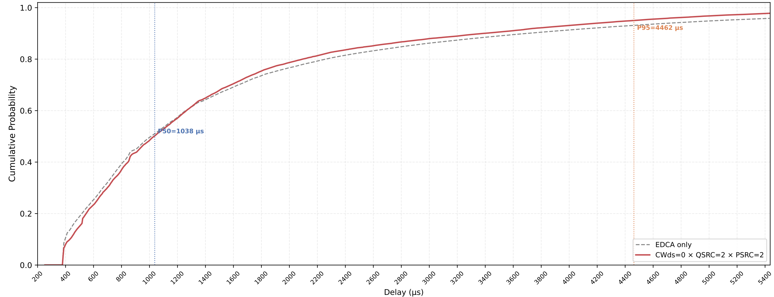
P-EDCA STA VO Delay CDF — CWds=0 × QSRC=2 × PSRC=2 nSta=30, nPedca=5, 0.5Mbps, avg of 10 runs
