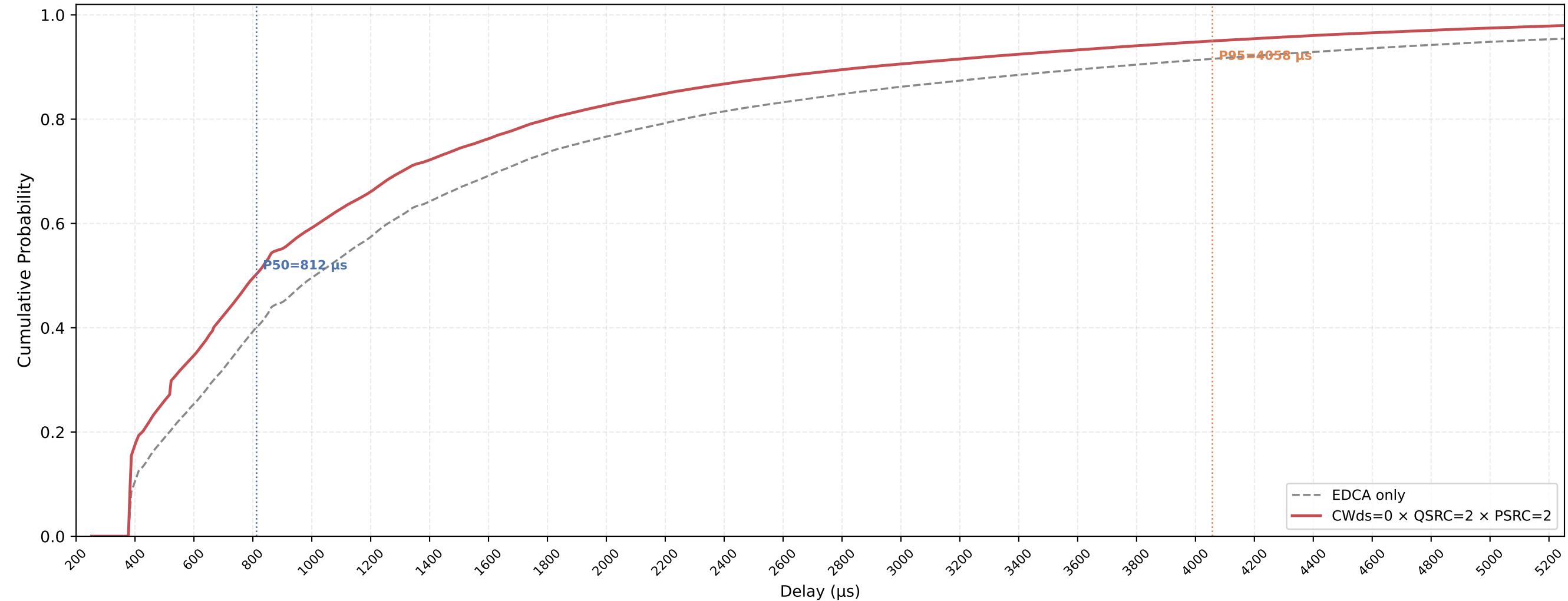
P-EDCA STA VO Delay CDF — CWds=0 × QSRC=2 × PSRC=2 nSta=30, nPedca=30, 0.5Mbps, avg of 10 runs
