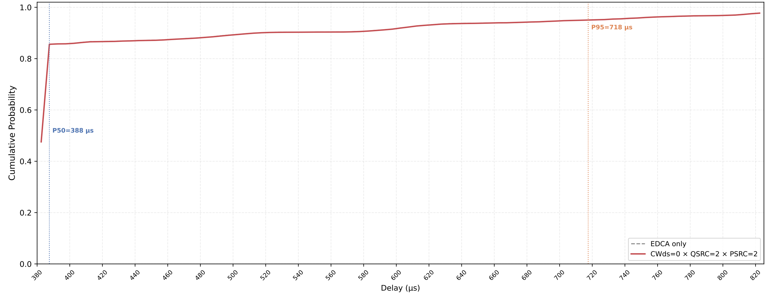
VO (all STAs) Delay CDF — CWds=0 × QSRC=2 × PSRC=2 nSta=30, nPedca=5, 0.1Mbps, avg of 10 runs
