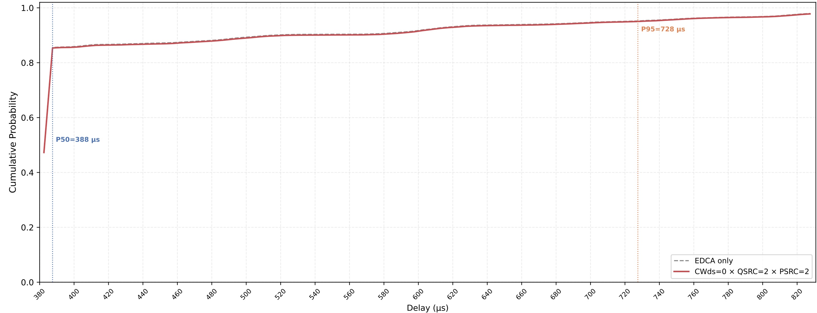
VO (all STAs) Delay CDF — CWds=0 × QSRC=2 × PSRC=2 nSta=30, nPedca=15, 0.1Mbps, avg of 10 runs
