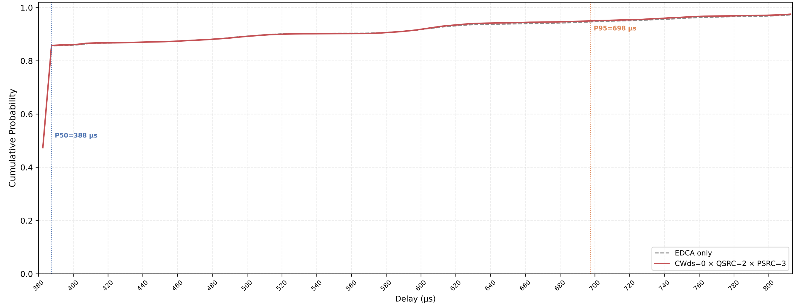
Legacy STA VO Delay CDF — CWds=0 × QSRC=2 × PSRC=3 nSta=30, nPedca=5, 0.1Mbps, avg of 10 runs
