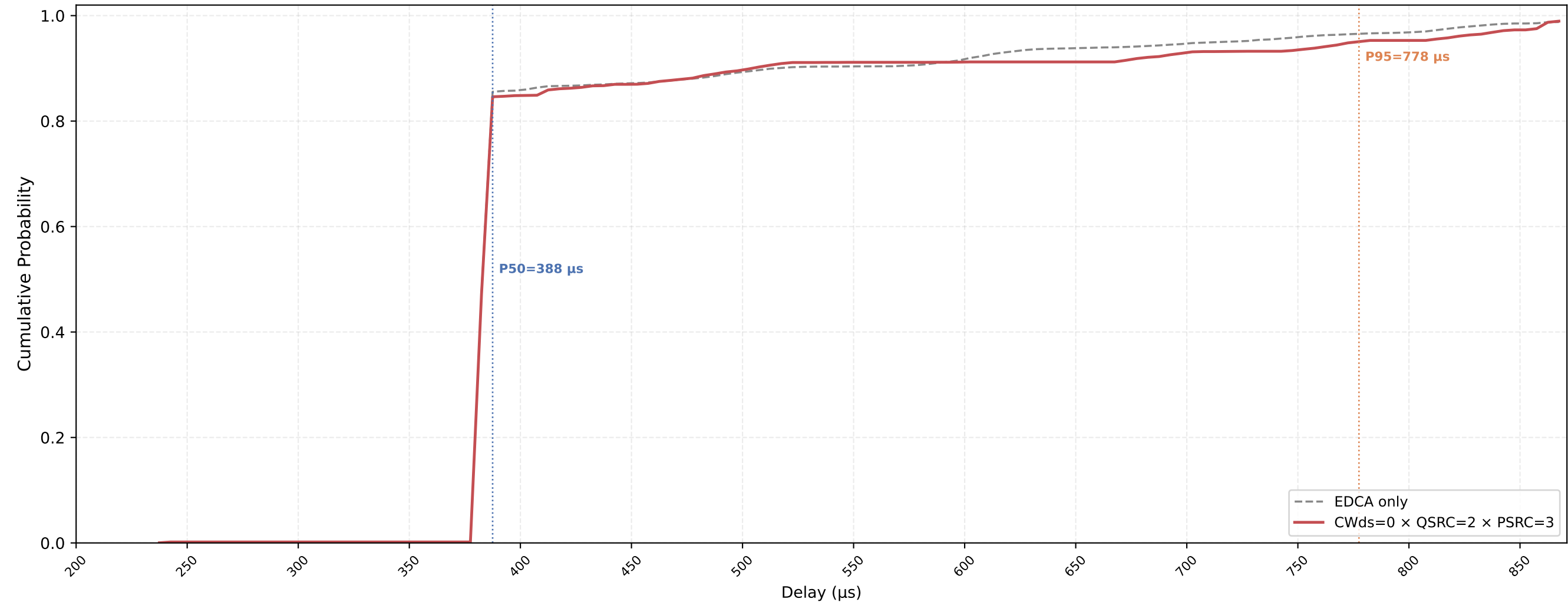
P-EDCA STA VO Delay CDF — CWds=0 × QSRC=2 × PSRC=3 nSta=30, nPedca=5, 0.1Mbps, avg of 10 runs
