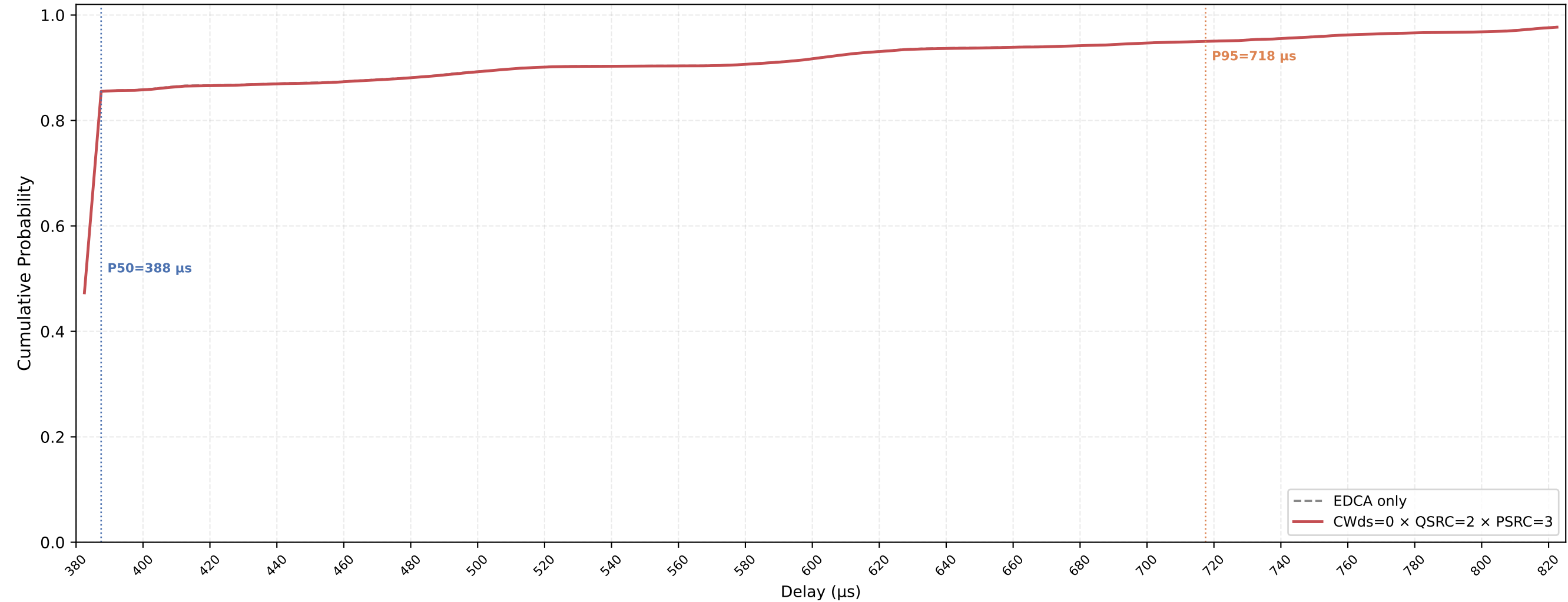
VO (all STAs) Delay CDF — CWds=0 × QSRC=2 × PSRC=3 nSta=30, nPedca=5, 0.1Mbps, avg of 10 runs
