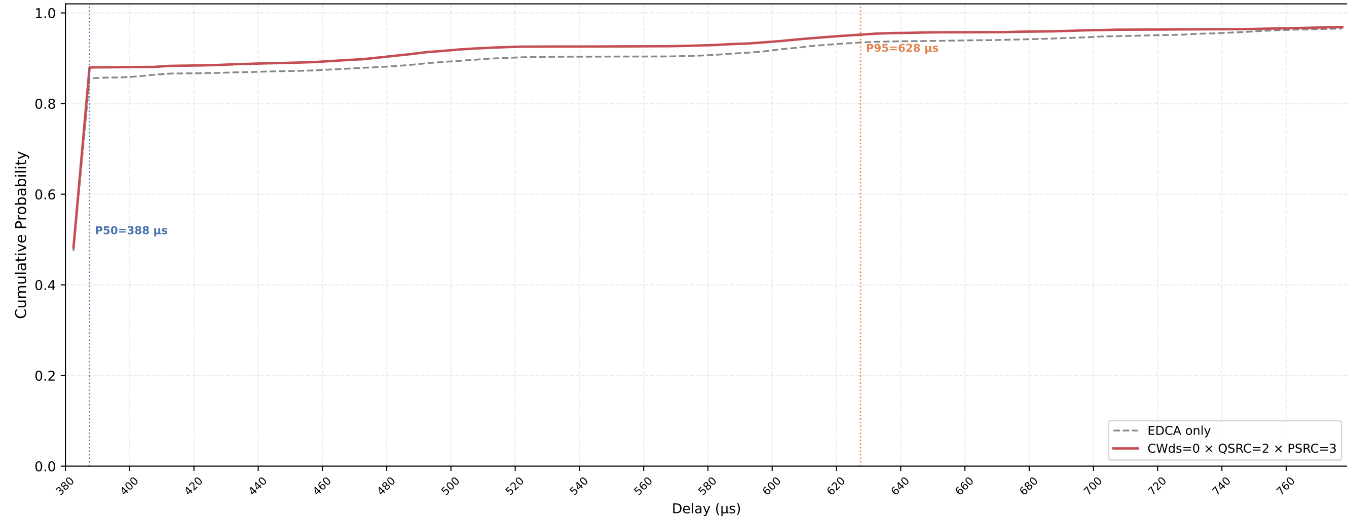
VO (all STAs) Delay CDF — CWds=0 × QSRC=2 × PSRC=3 nSta=30, nPedca=30, 0.1Mbps, avg of 10 runs
