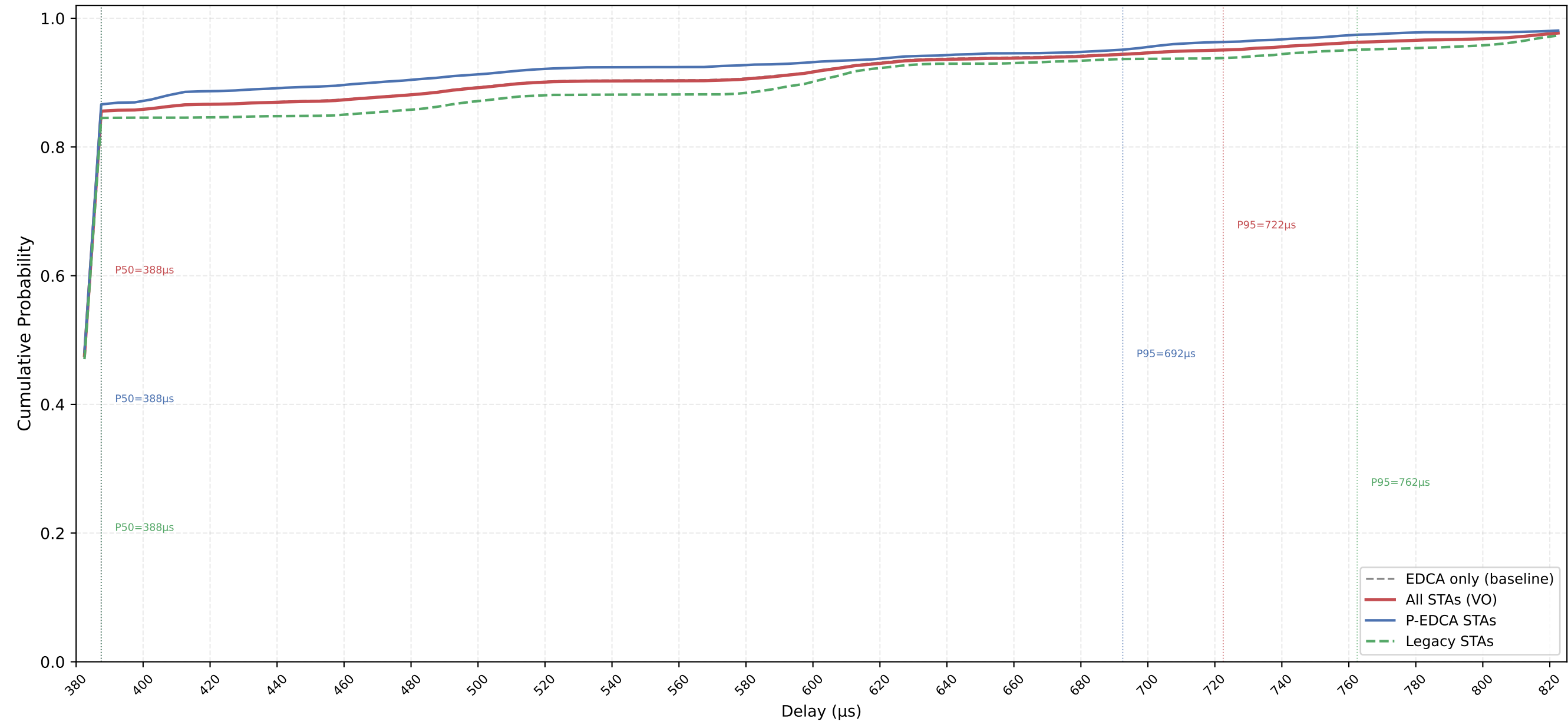
VO Delay CDF — P-EDCA / Legacy / All | CWds=0 × QSRC=3 × PSRC=1 nSta=30, nPedca=15/30, 0.1Mbps, avg of 10 runs
