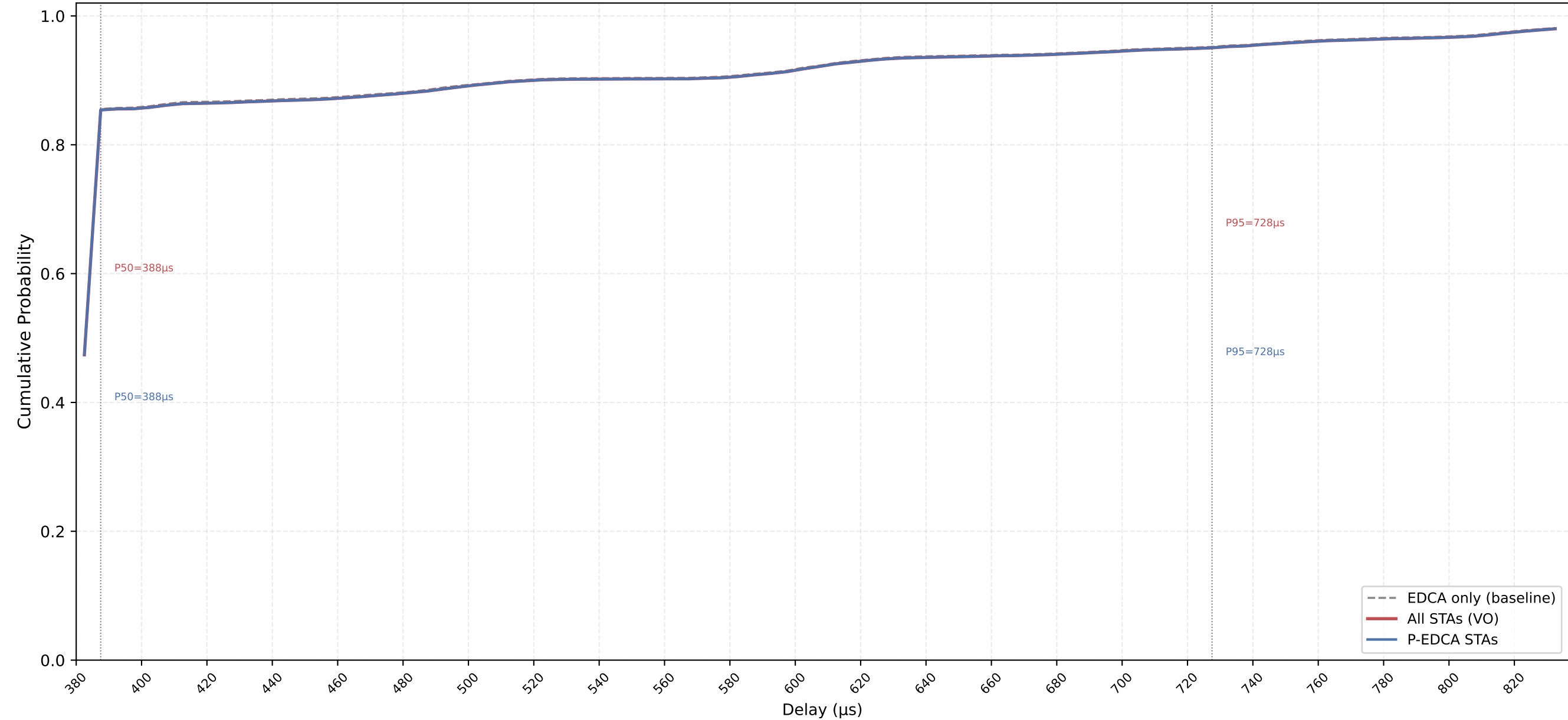
VO Delay CDF — P-EDCA / Legacy / All | CWds=0 × QSRC=3 × PSRC=1 nSta=30, nPedca=30/30, 0.1Mbps, avg of 10 runs
