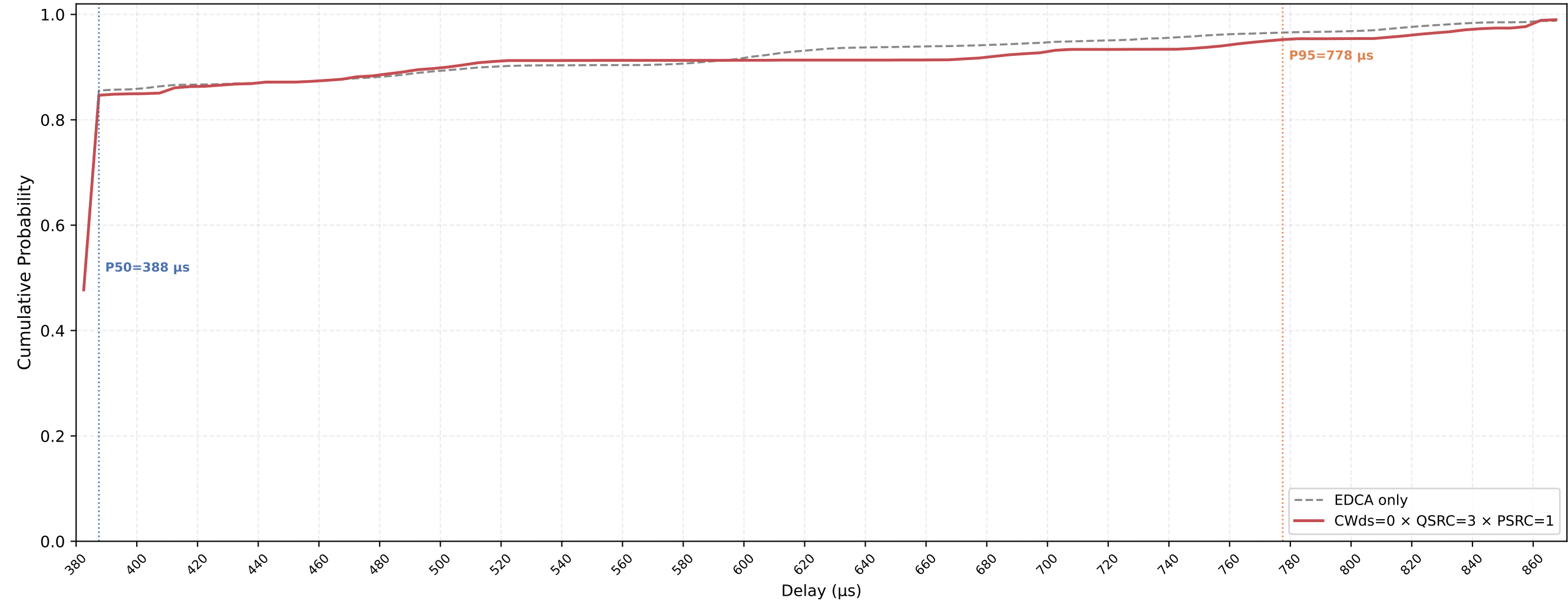
P-EDCA STA VO Delay CDF — CWds=0 × QSRC=3 × PSRC=1 nSta=30, nPedca=5, 0.1Mbps, avg of 10 runs
