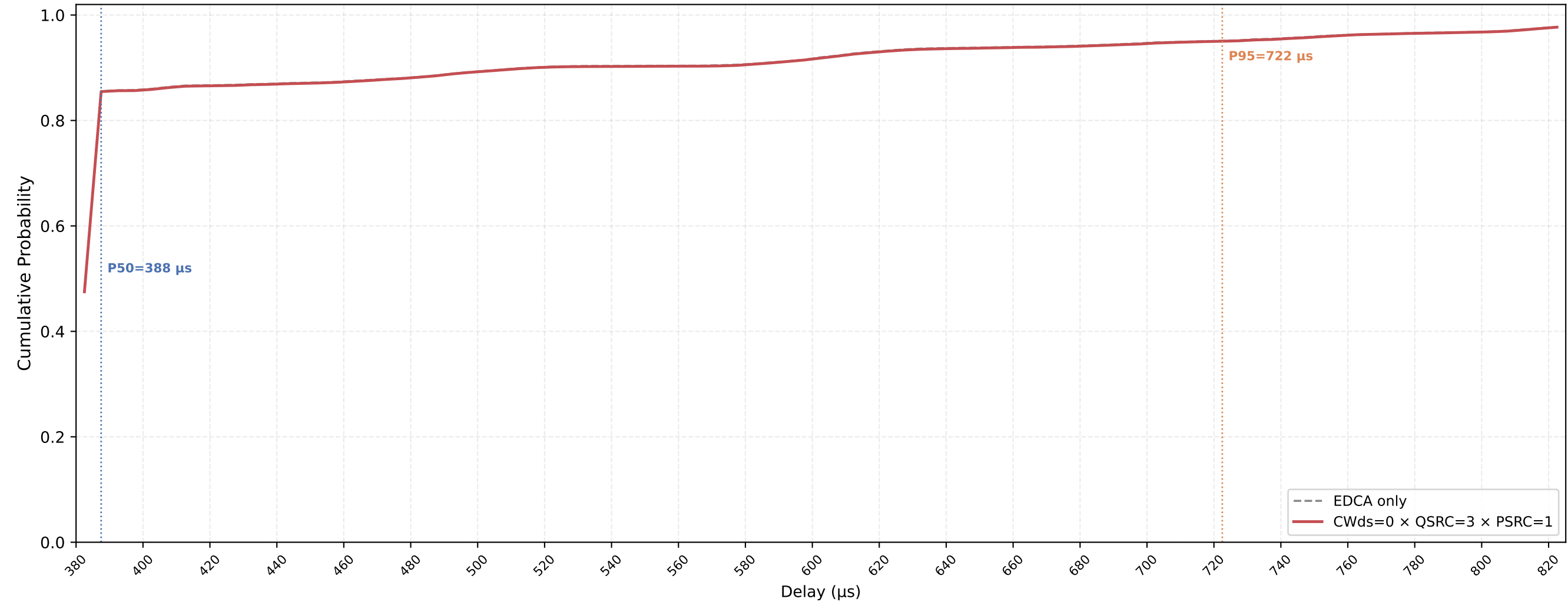
VO (all STAs) Delay CDF — CWds=0 × QSRC=3 × PSRC=1 nSta=30, nPedca=5, 0.1Mbps, avg of 10 runs
