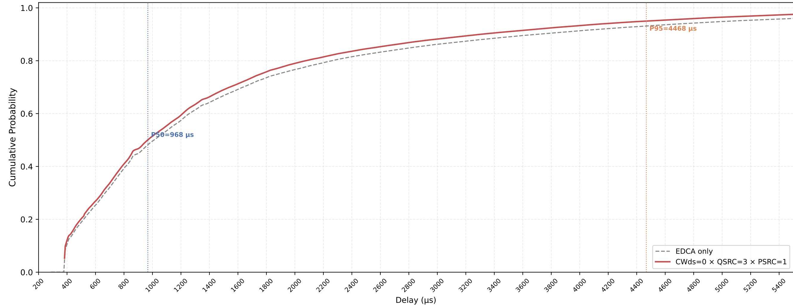
VO (all STAs) Delay CDF — CWds=0 × QSRC=3 × PSRC=1 nSta=30, nPedca=30, 0.5Mbps, avg of 10 runs
