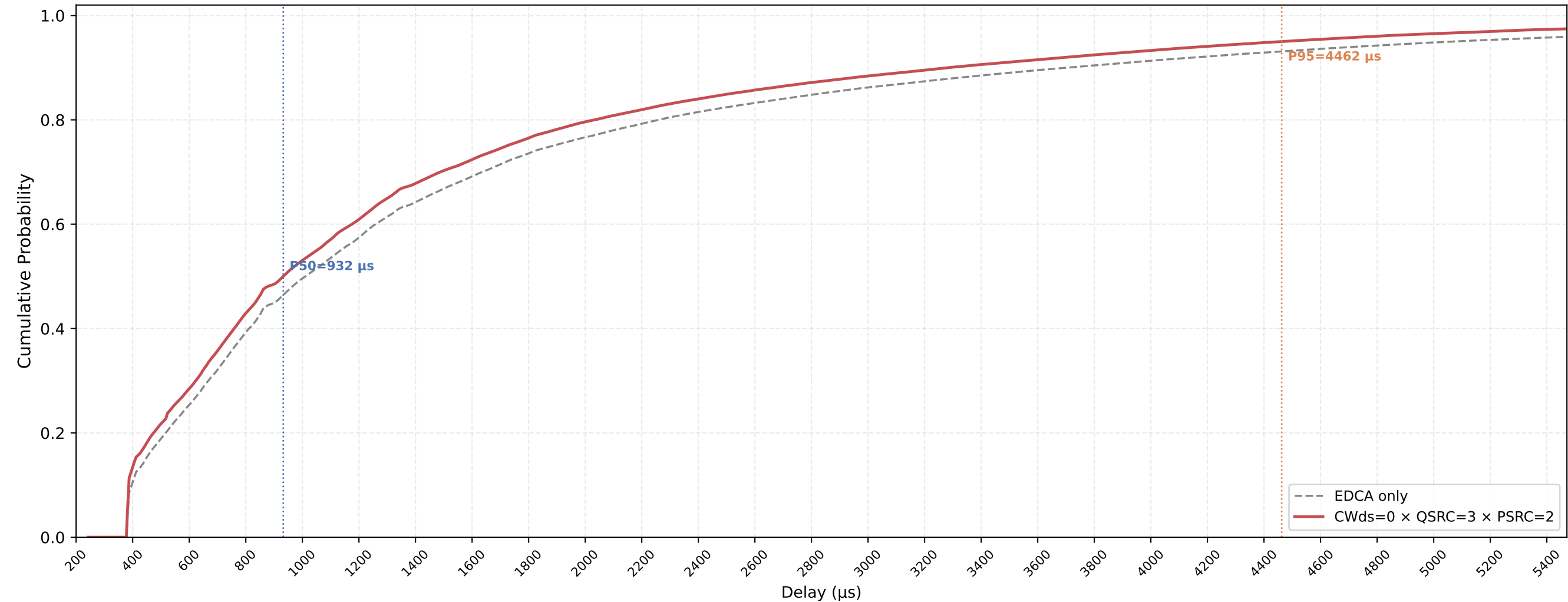
P-EDCA STA VO Delay CDF — CWds=0 × QSRC=3 × PSRC=2 nSta=30, nPedca=30, 0.5Mbps, avg of 10 runs
