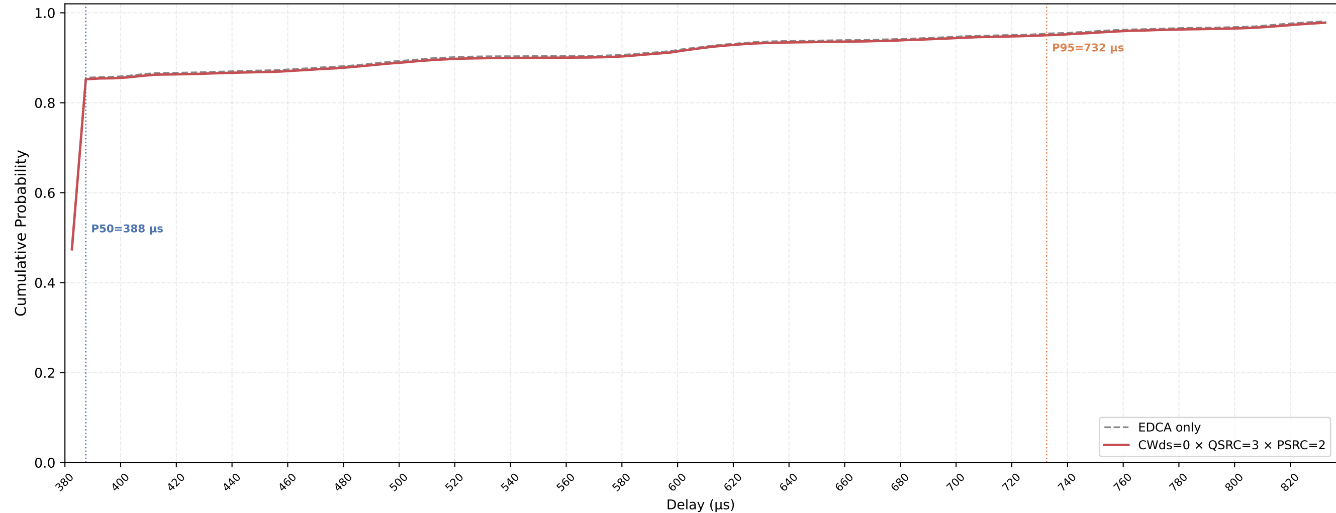
VO (all STAs) Delay CDF — CWds=0 × QSRC=3 × PSRC=2 nSta=30, nPedca=30, 0.1Mbps, avg of 10 runs
