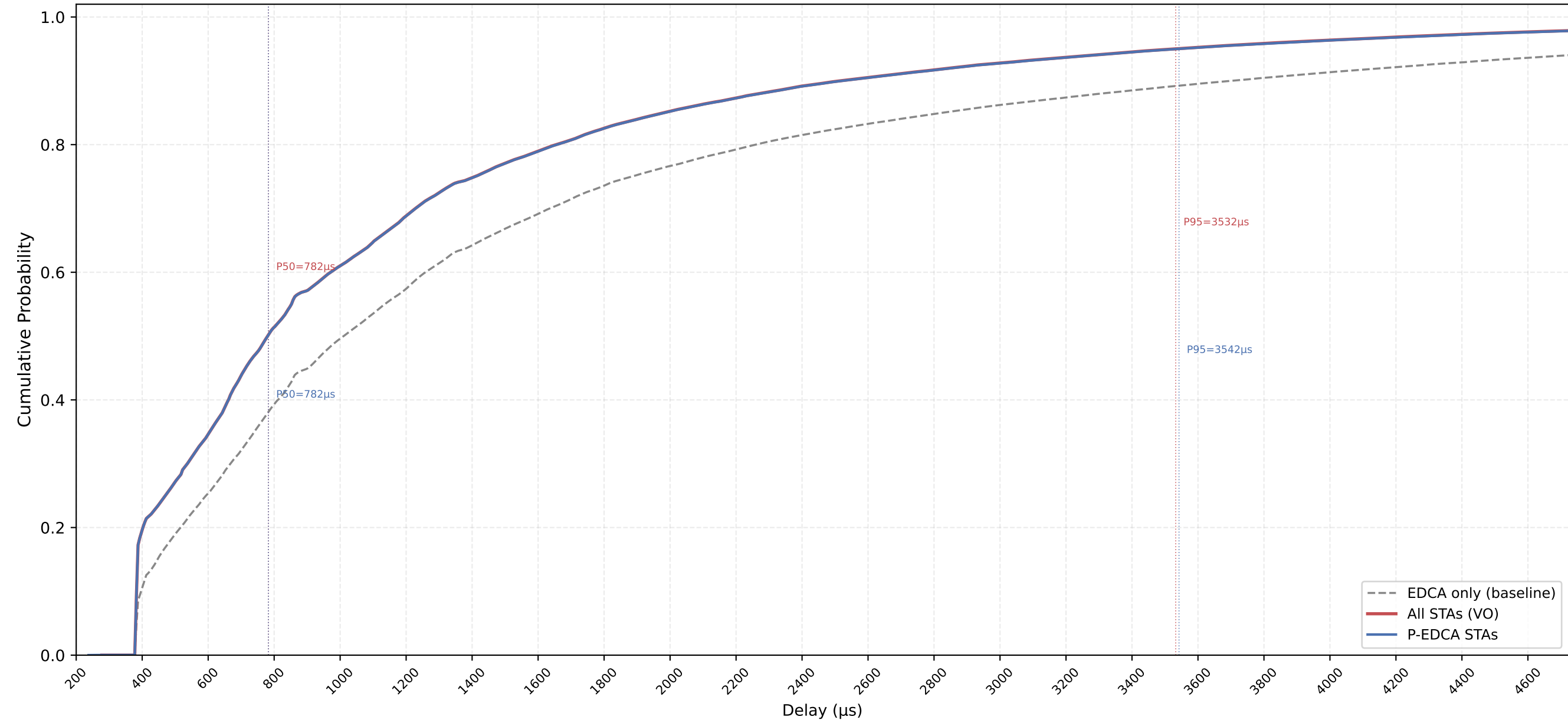
VO Delay CDF — P-EDCA / Legacy / All | CWds=0 × QSRC=3 × PSRC=3 nSta=30, nPedca=30/30, 0.5Mbps, avg of 10 runs
