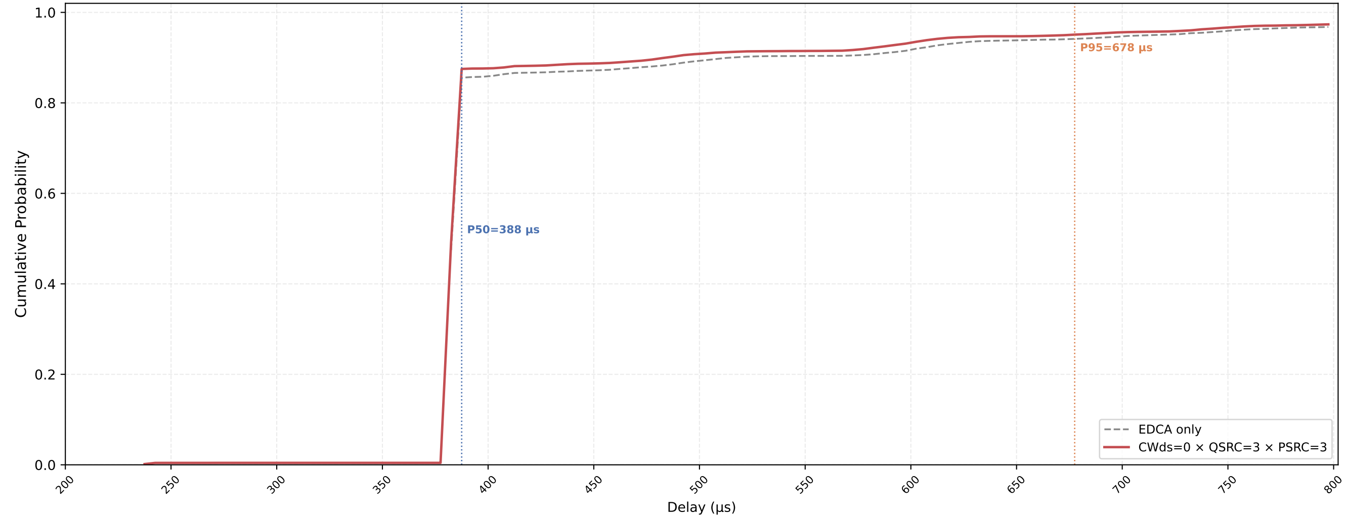
P-EDCA STA VO Delay CDF — CWds=0 × QSRC=3 × PSRC=3 nSta=30, nPedca=30, 0.1Mbps, avg of 10 runs
