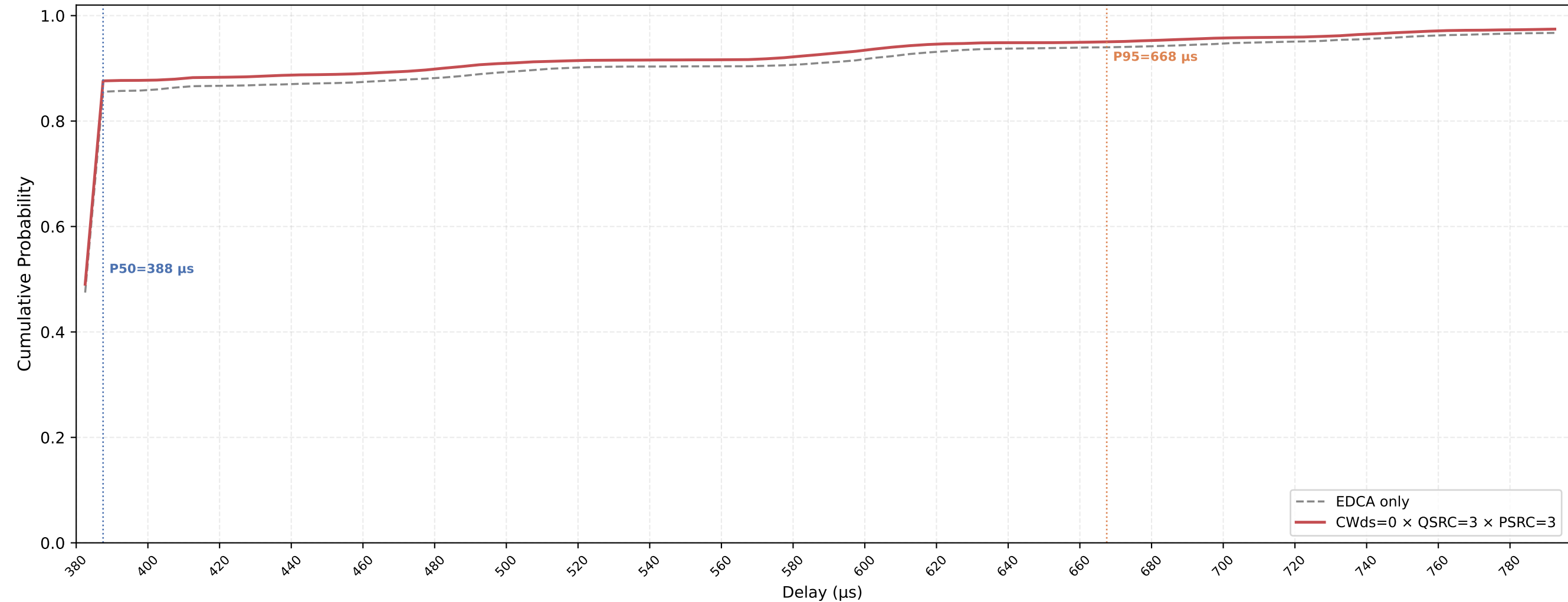
VO (all STAs) Delay CDF — CWds=0 × QSRC=3 × PSRC=3 nSta=30, nPedca=30, 0.1Mbps, avg of 10 runs
