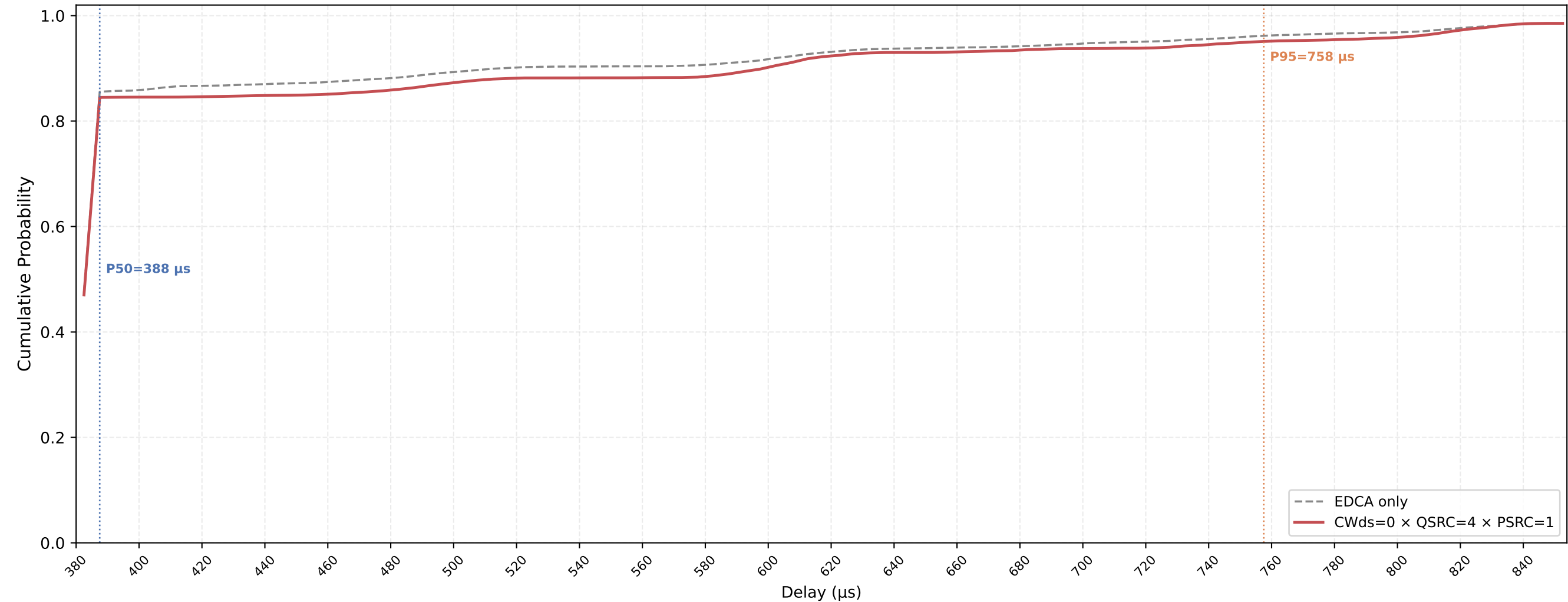
Legacy STA VO Delay CDF — CWds=0 × QSRC=4 × PSRC=1 nSta=30, nPedca=15, 0.1Mbps, avg of 10 runs
