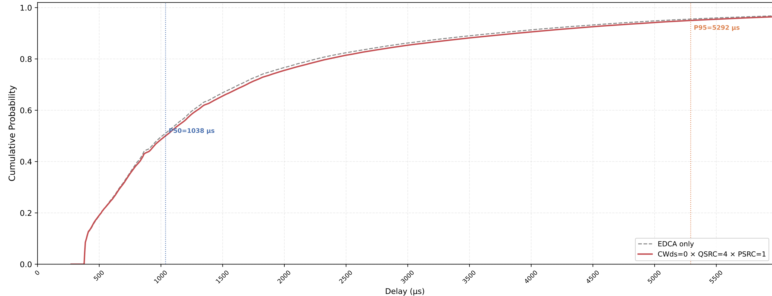
VO (all STAs) Delay CDF — CWds=0 × QSRC=4 × PSRC=1 nSta=30, nPedca=30, 0.5Mbps, avg of 10 runs
