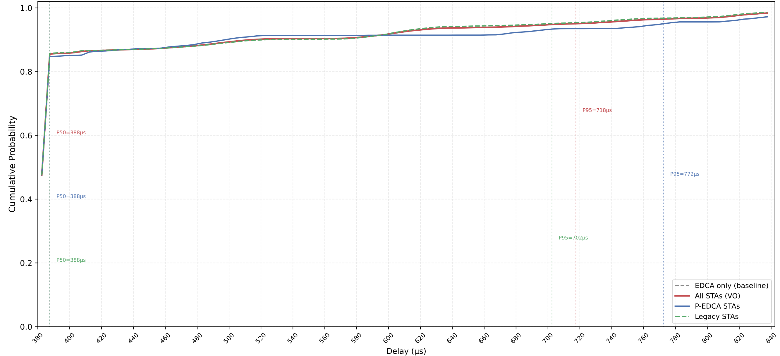
VO Delay CDF — P-EDCA / Legacy / All | CWds=0 × QSRC=4 × PSRC=2 nSta=30, nPedca=5/30, 0.1Mbps, avg of 10 runs
